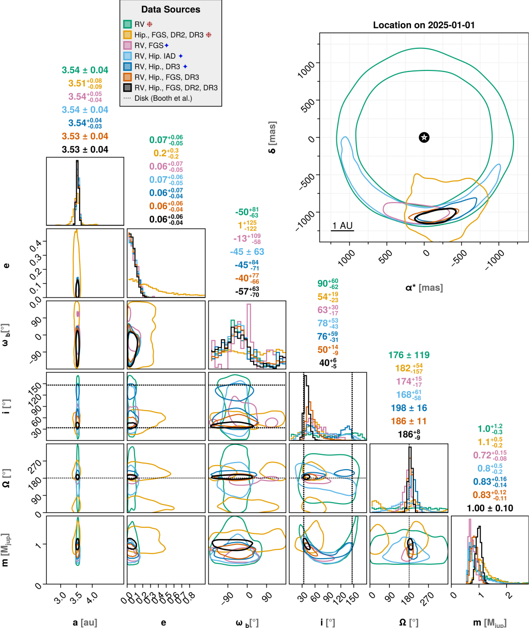
Figure 2. from William Thompson et al 2025 Astron. J. 170 doi:10.3847/1538-3881/ae0cbd https://dx.doi.org/10.3847/1538-3881/ae0cbd © 2025. The Author(s). Published by the American Astronomical Society.
