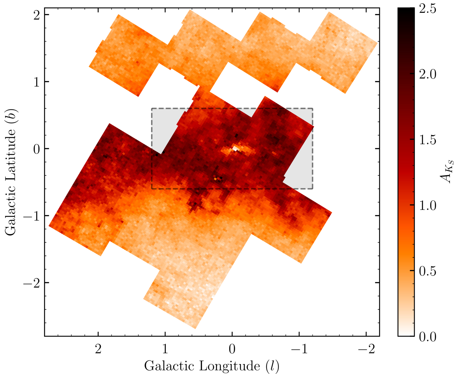
Figure 7. from Aiden S. Zelakiewicz et al 2025 Astron. J. 170 doi:10.3847/1538-3881/ae0c0b https://dx.doi.org/10.3847/1538-3881/ae0c0b © 2025. The Author(s). Published by the American Astronomical Society.
