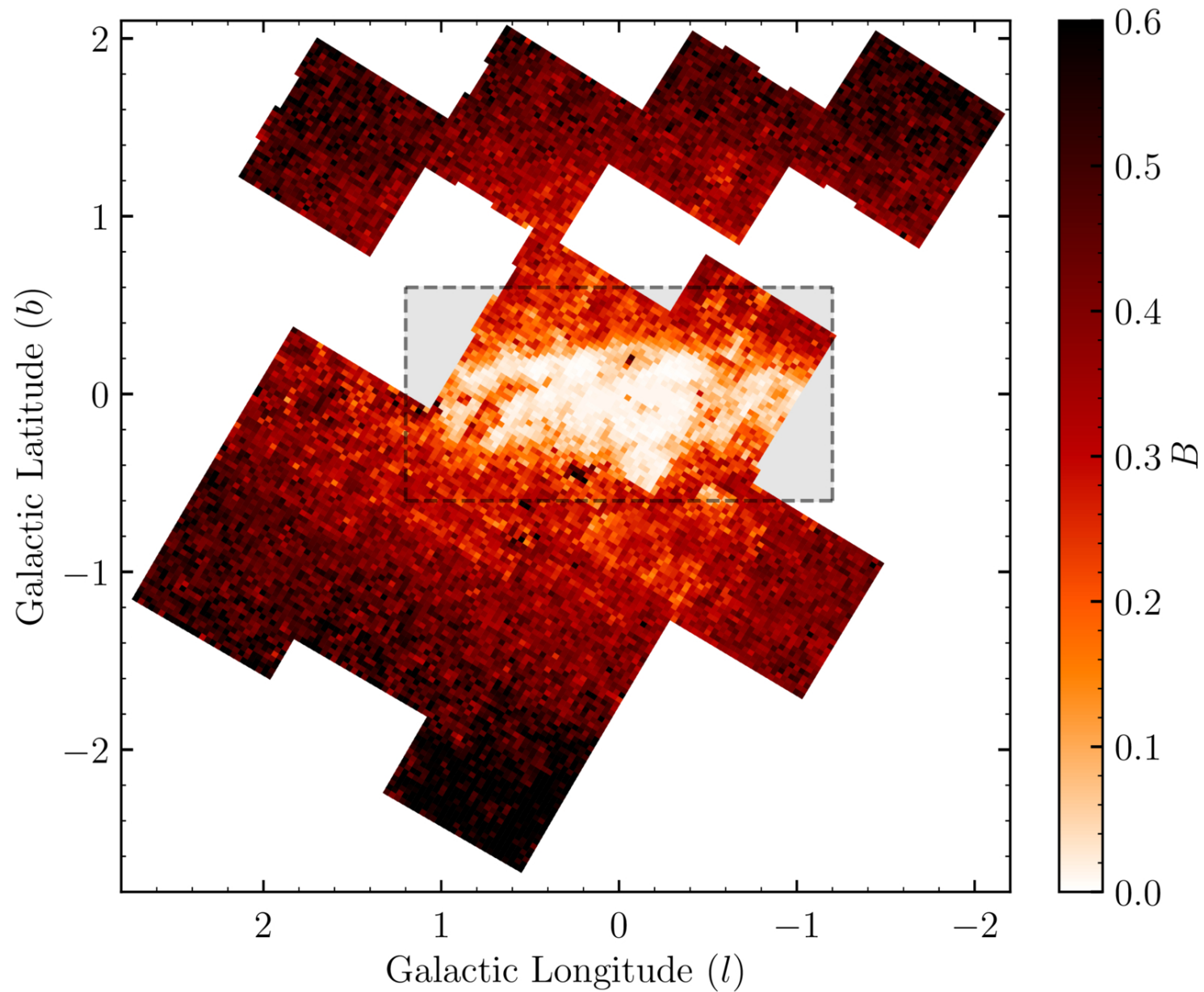
Figure 6. from Aiden S. Zelakiewicz et al 2025 Astron. J. 170 doi:10.3847/1538-3881/ae0c0b https://dx.doi.org/10.3847/1538-3881/ae0c0b © 2025. The Author(s). Published by the American Astronomical Society.
