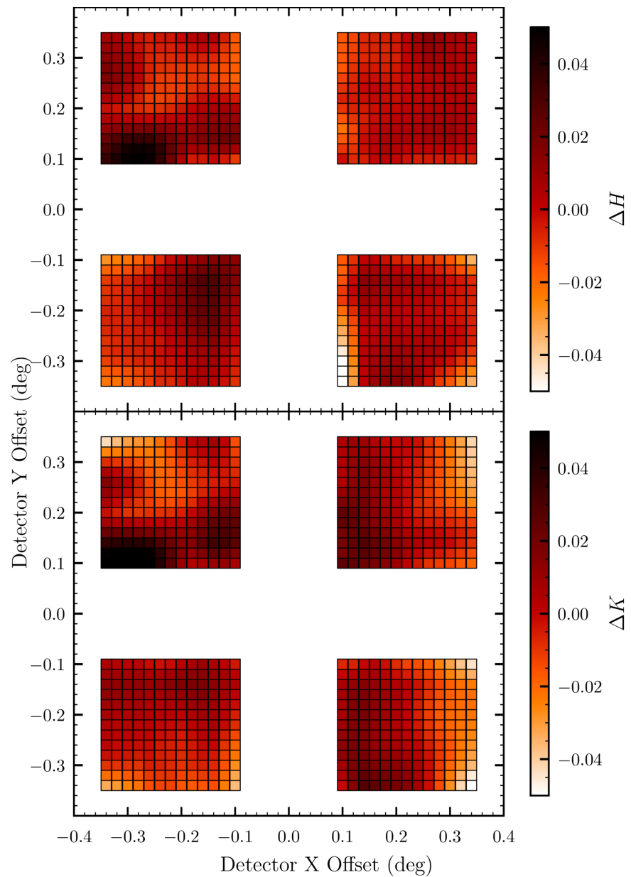
Figure 2. from Aiden S. Zelakiewicz et al 2025 Astron. J. 170 doi:10.3847/1538-3881/ae0c0b https://dx.doi.org/10.3847/1538-3881/ae0c0b © 2025. The Author(s). Published by the American Astronomical Society.
