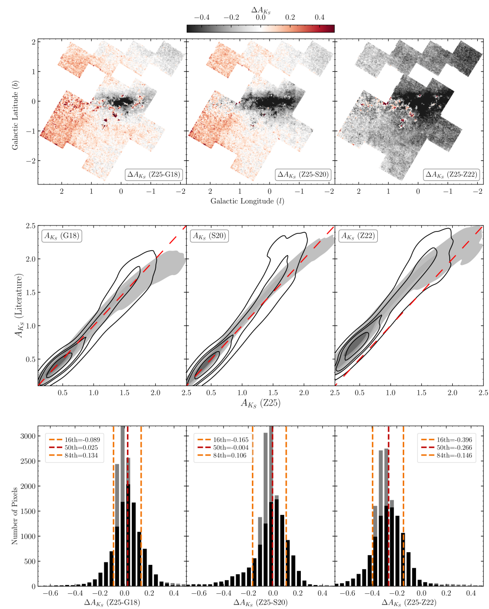
Figure 13. from Aiden S. Zelakiewicz et al 2025 Astron. J. 170 doi:10.3847/1538-3881/ae0c0b https://dx.doi.org/10.3847/1538-3881/ae0c0b © 2025. The Author(s). Published by the American Astronomical Society.
