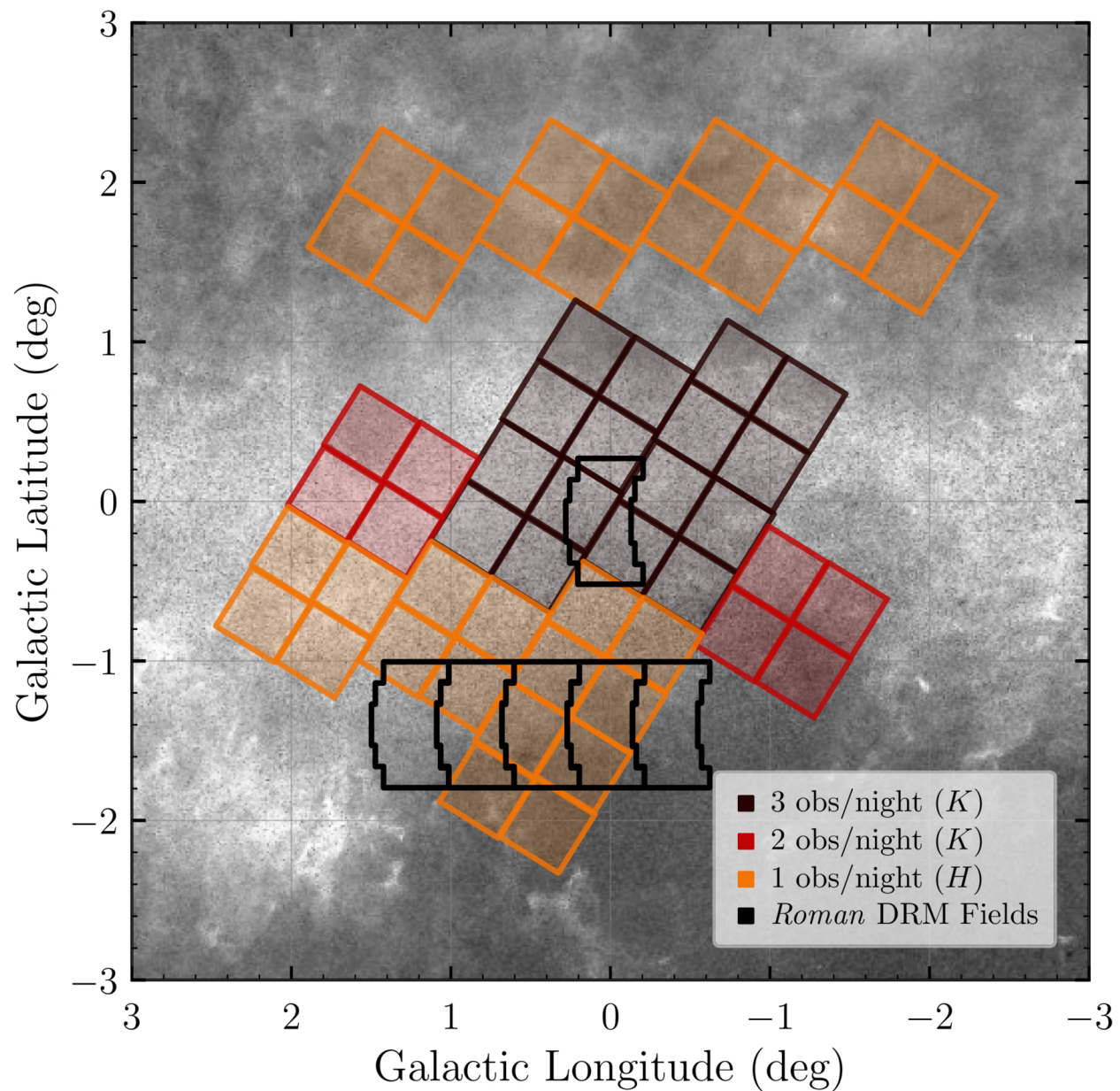
Figure 1. from Aiden S. Zelakiewicz et al 2025 Astron. J. 170 doi:10.3847/1538-3881/ae0c0b https://dx.doi.org/10.3847/1538-3881/ae0c0b © 2025. The Author(s). Published by the American Astronomical Society.
