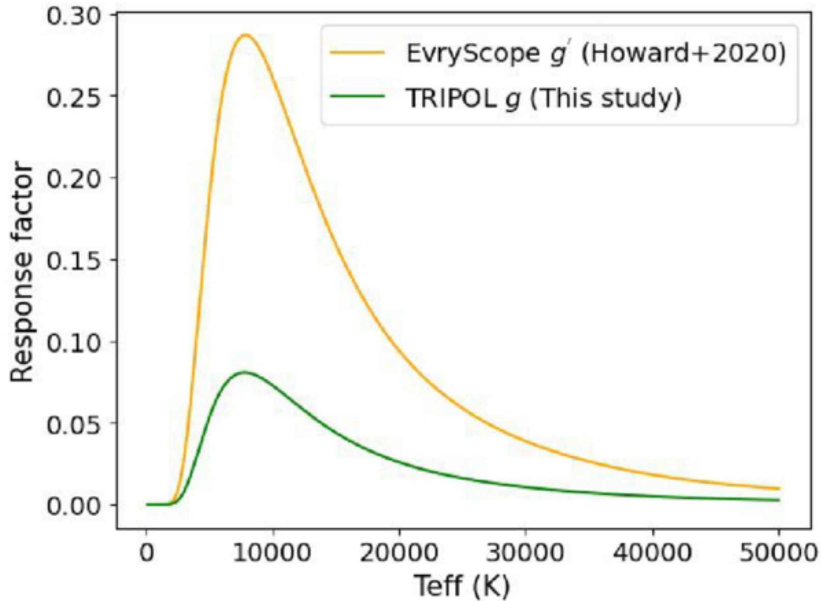
Figure 6. from Chia-Lung Lin et al 2025 Astron. J. 170 doi:10.3847/1538-3881/ae0c0a https://dx.doi.org/10.3847/1538-3881/ae0c0a © 2025. The Author(s). Published by the American Astronomical Society.
