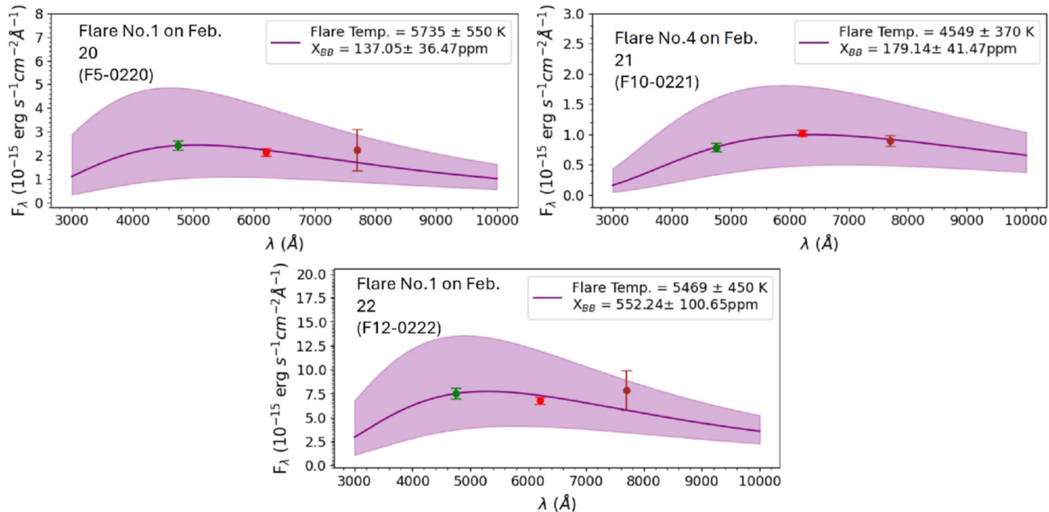
Figure 4. from Chia-Lung Lin et al 2025 Astron. J. 170 doi:10.3847/1538-3881/ae0c0a https://dx.doi.org/10.3847/1538-3881/ae0c0a © 2025. The Author(s). Published by the American Astronomical Society.
