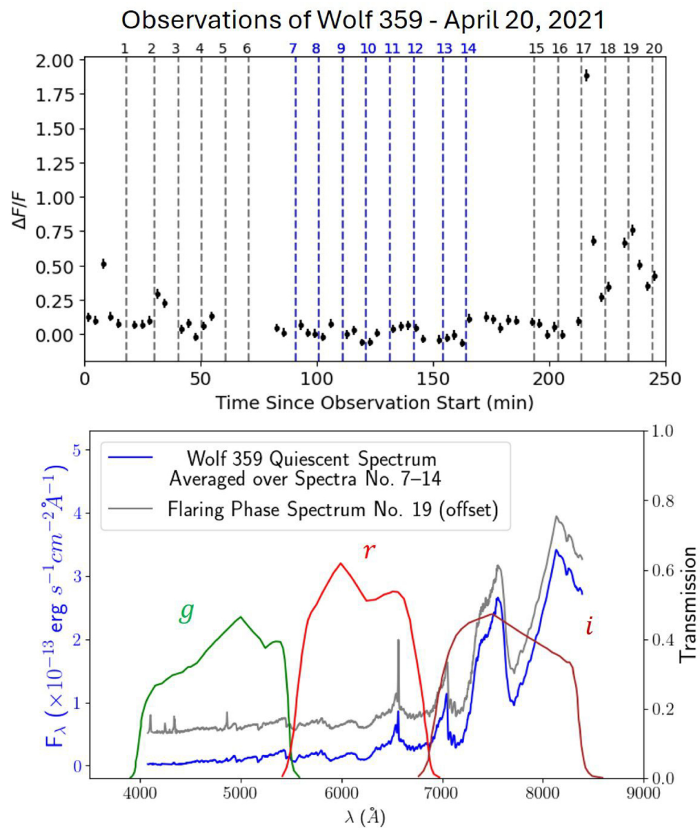
Figure 3. from Chia-Lung Lin et al 2025 Astron. J. 170 doi:10.3847/1538-3881/ae0c0a https://dx.doi.org/10.3847/1538-3881/ae0c0a © 2025. The Author(s). Published by the American Astronomical Society.
