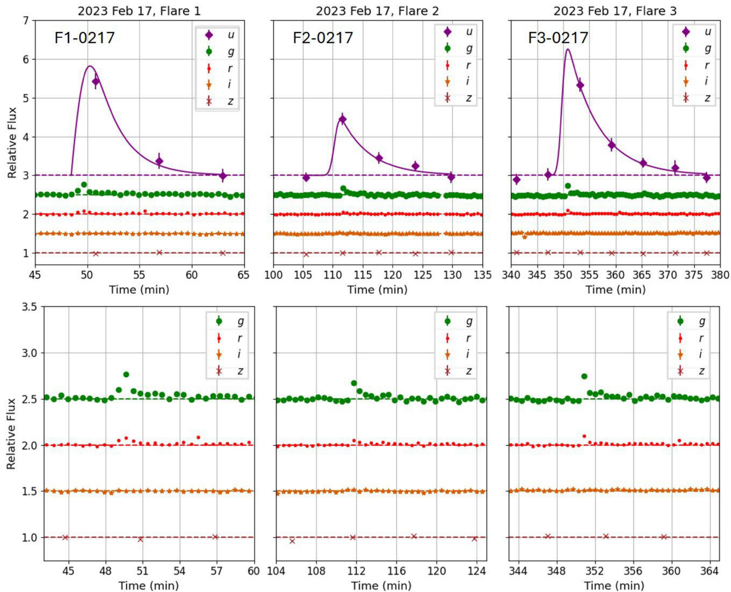
Figure 2. from Chia-Lung Lin et al 2025 Astron. J. 170 doi:10.3847/1538-3881/ae0c0a https://dx.doi.org/10.3847/1538-3881/ae0c0a © 2025. The Author(s). Published by the American Astronomical Society.
