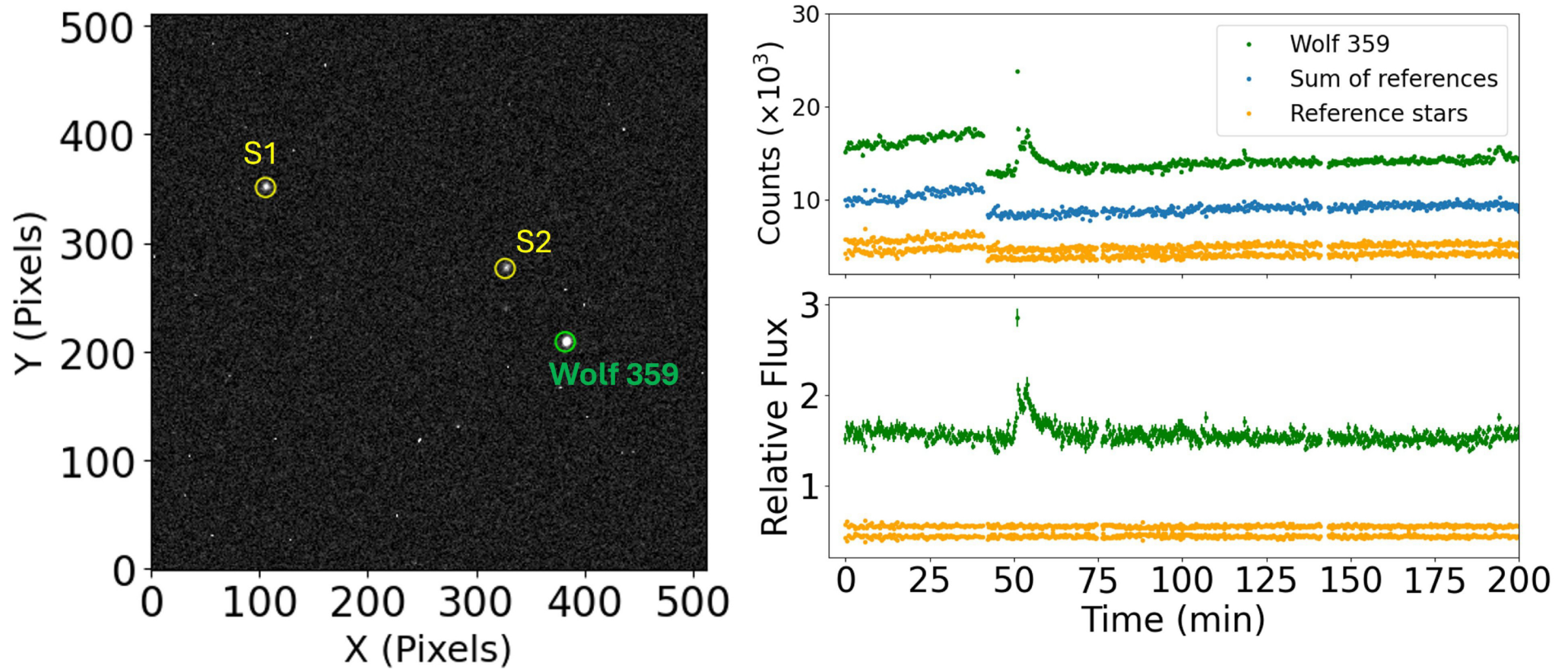
Figure 1. from Chia-Lung Lin et al 2025 Astron. J. 170 doi:10.3847/1538-3881/ae0c0a https://dx.doi.org/10.3847/1538-3881/ae0c0a © 2025. The Author(s). Published by the American Astronomical Society.
