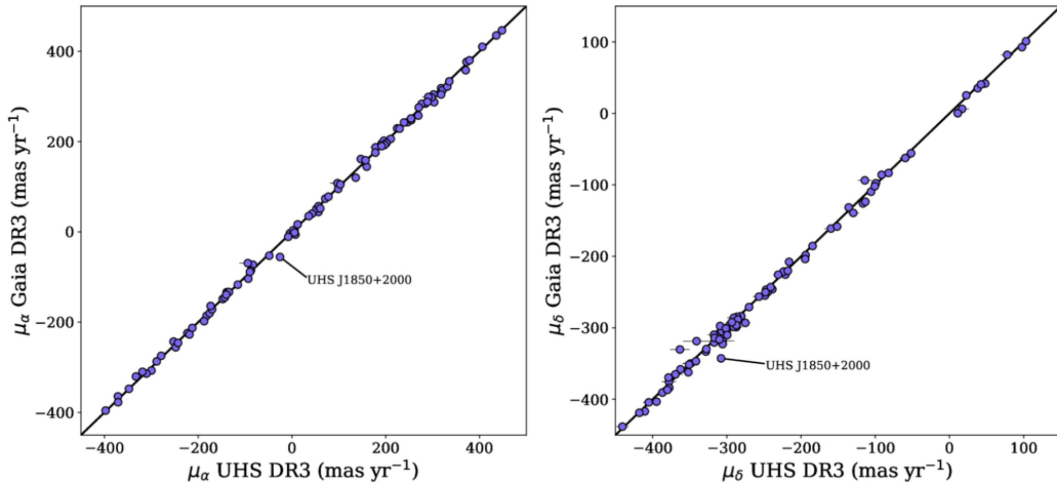
Figure 3. from Wings Zhang et al 2025 Astron. J. 170 doi:10.3847/1538-3881/ae0ad5 https://dx.doi.org/10.3847/1538-3881/ae0ad5 © 2025. The Author(s). Published by the American Astronomical Society.
