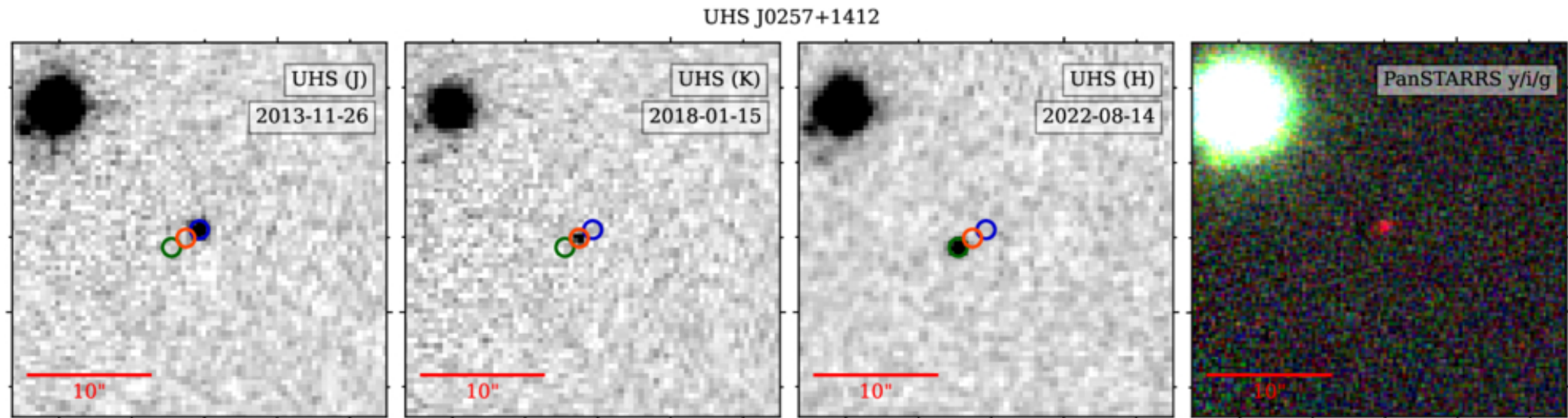
Figure 1. from Wings Zhang et al 2025 Astron. J. 170 doi:10.3847/1538-3881/ae0ad5 https://dx.doi.org/10.3847/1538-3881/ae0ad5 © 2025. The Author(s). Published by the American Astronomical Society.
