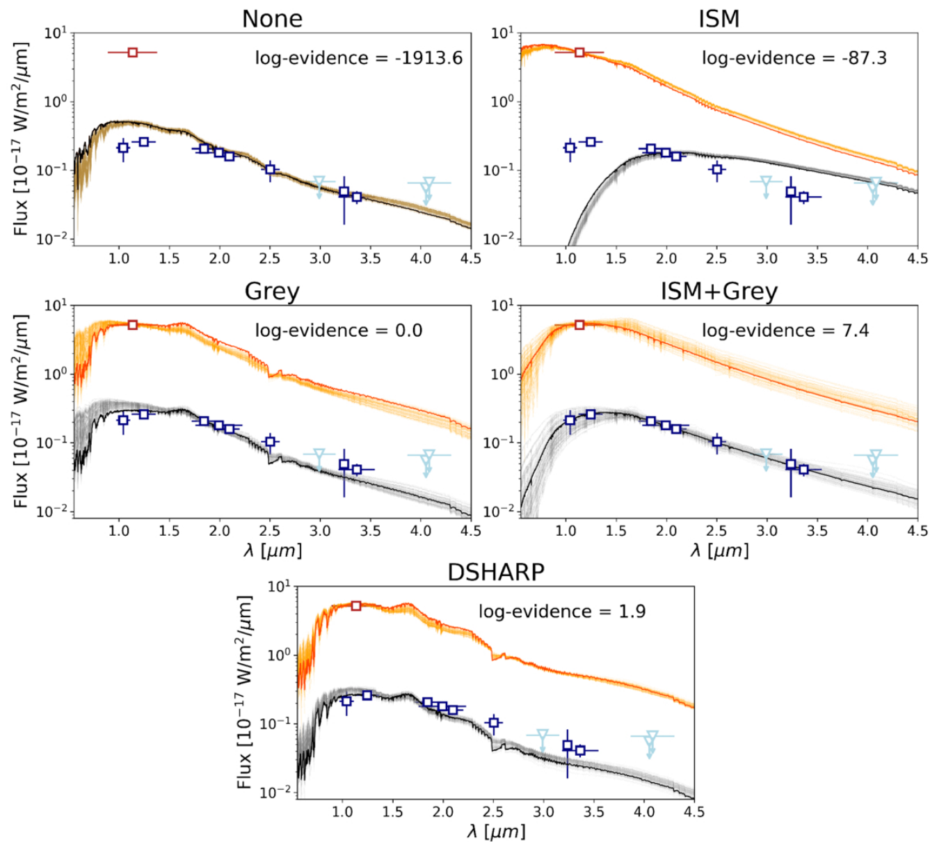
Figure 8. from Gabriele Cugno et al 2025 Astron. J. 170 doi:10.3847/1538-3881/ae0acd https://dx.doi.org/10.3847/1538-3881/ae0acd © 2025. The Author(s). Published by the American Astronomical Society.
