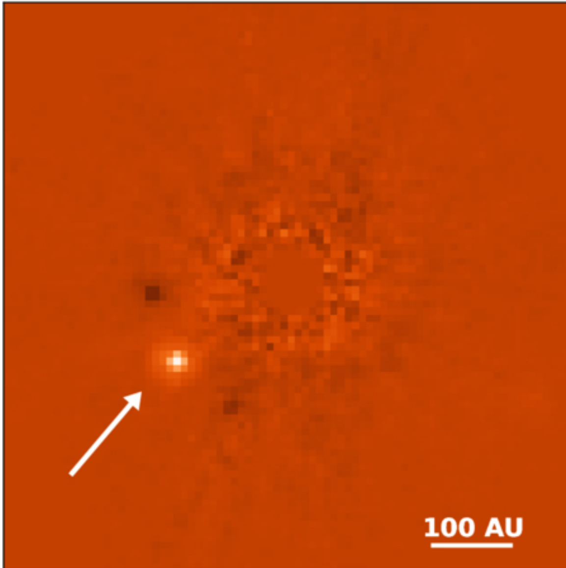
Figure 4. from Gabriele Cugno et al 2025 Astron. J. 170 doi:10.3847/1538-3881/ae0acd https://dx.doi.org/10.3847/1538-3881/ae0acd © 2025. The Author(s). Published by the American Astronomical Society.
