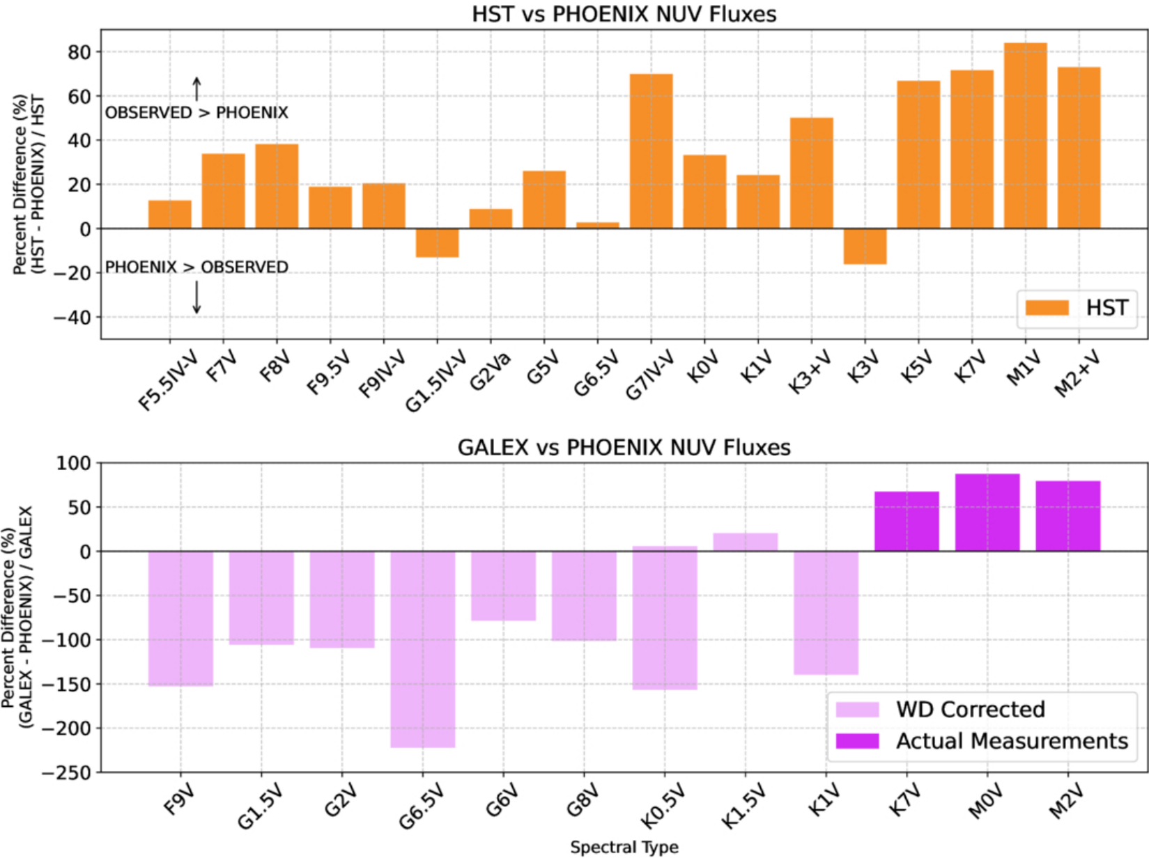
Figure 9. from Sarah Peacock et al 2025 Astron. J. 170 doi:10.3847/1538-3881/ae0a2f https://dx.doi.org/10.3847/1538-3881/ae0a2f © 2025. The Author(s). Published by the American Astronomical Society.
