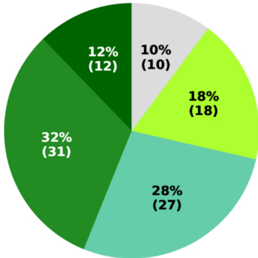
Figure 4. from Sarah Peacock et al 2025 Astron. J. 170 doi:10.3847/1538-3881/ae0a2f https://dx.doi.org/10.3847/1538-3881/ae0a2f © 2025. The Author(s). Published by the American Astronomical Society.
