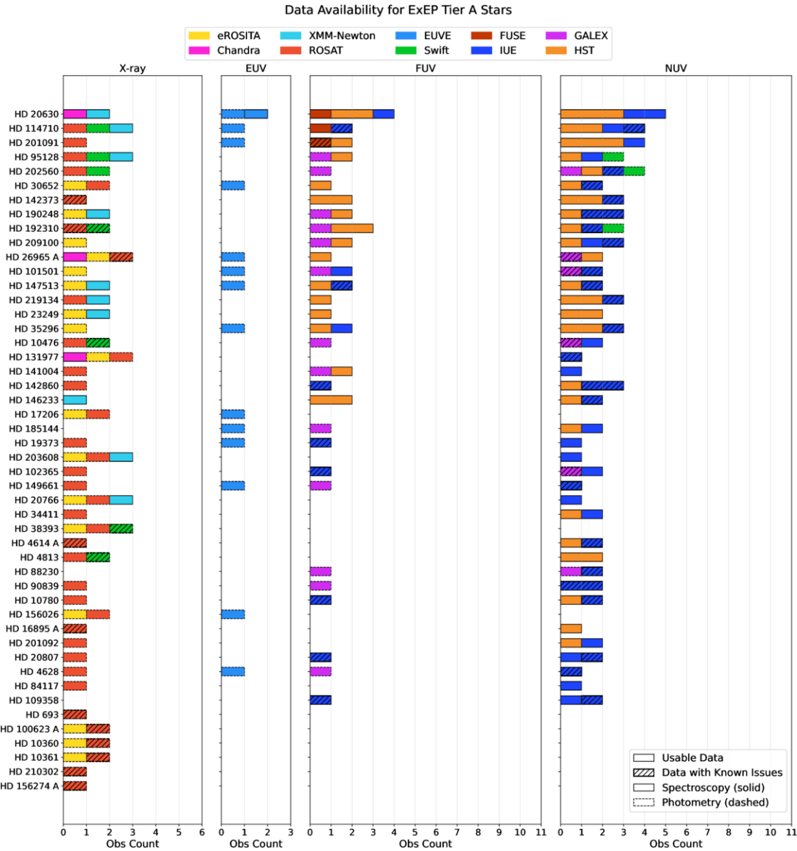
Figure 2. from Sarah Peacock et al 2025 Astron. J. 170 doi:10.3847/1538-3881/ae0a2f https://dx.doi.org/10.3847/1538-3881/ae0a2f © 2025. The Author(s). Published by the American Astronomical Society.
