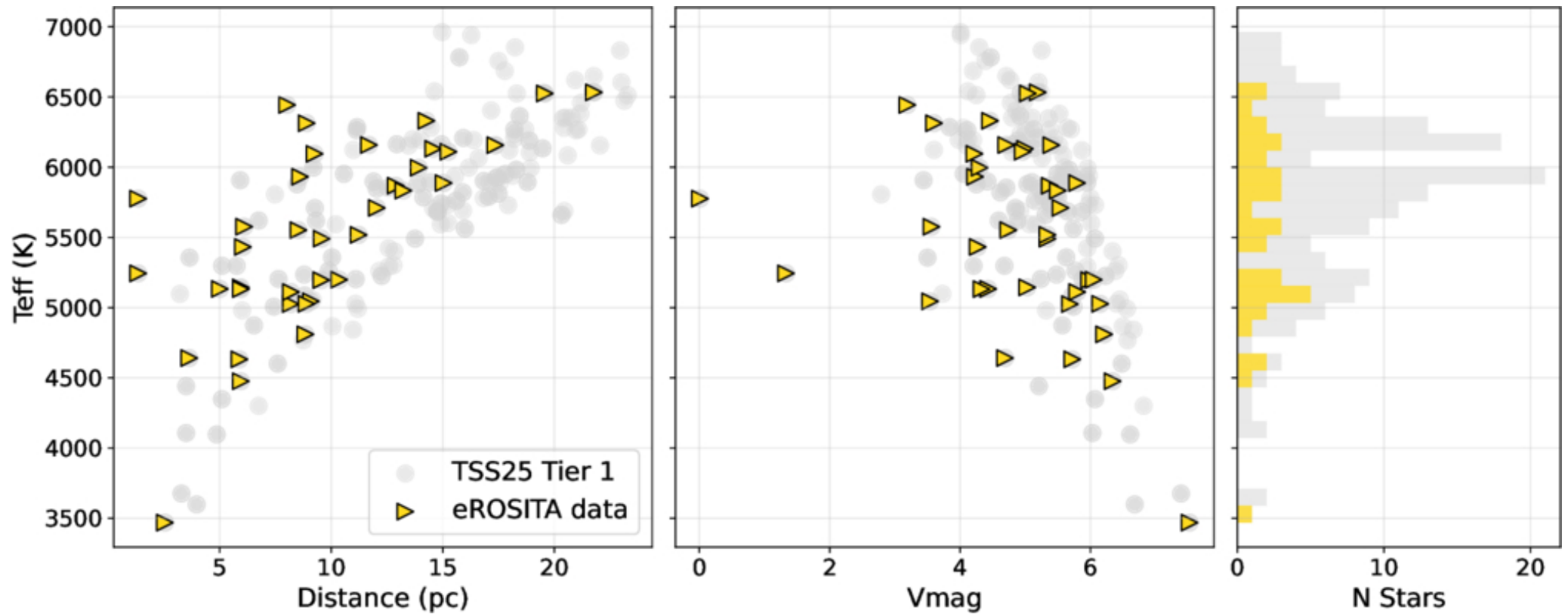
Figure 13. from Sarah Peacock et al 2025 Astron. J. 170 doi:10.3847/1538-3881/ae0a2f https://dx.doi.org/10.3847/1538-3881/ae0a2f © 2025. The Author(s). Published by the American Astronomical Society.
