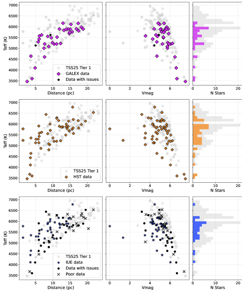
Figure 11. from Sarah Peacock et al 2025 Astron. J. 170 doi:10.3847/1538-3881/ae0a2f https://dx.doi.org/10.3847/1538-3881/ae0a2f © 2025. The Author(s). Published by the American Astronomical Society.
