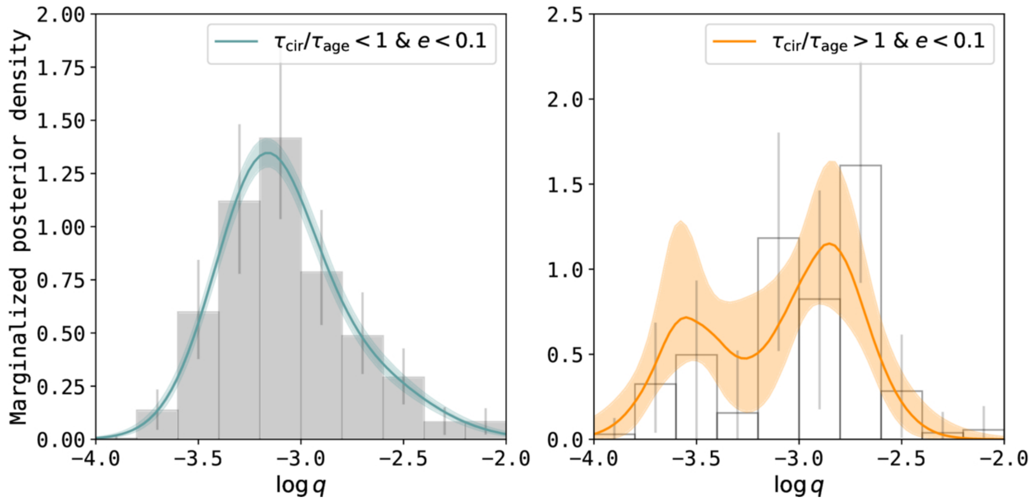
Figure 5. from Yugo Kawai et al 2025 Astron. J. 170 doi:10.3847/1538-3881/ae0a11 https://dx.doi.org/10.3847/1538-3881/ae0a11 © 2025. The Author(s). Published by the American Astronomical Society.
