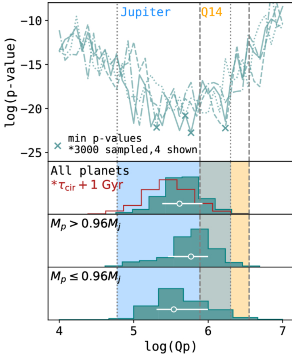
Figure 1. from Yugo Kawai et al 2025 Astron. J. 170 doi:10.3847/1538-3881/ae0a11 https://dx.doi.org/10.3847/1538-3881/ae0a11 © 2025. The Author(s). Published by the American Astronomical Society.
