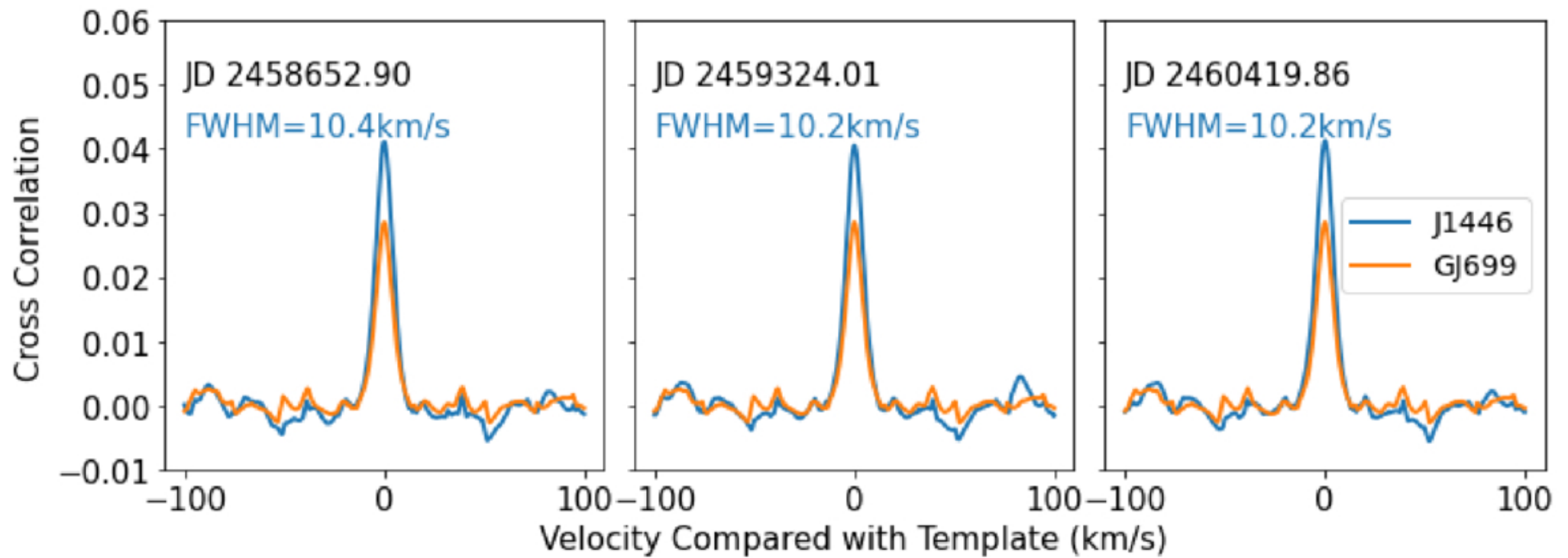
Figure 7. from Taichi Uyama et al 2025 Astron. J. 170 doi:10.3847/1538-3881/ae08b6 https://dx.doi.org/10.3847/1538-3881/ae08b6 © 2025. The Author(s). Published by the American Astronomical Society.
