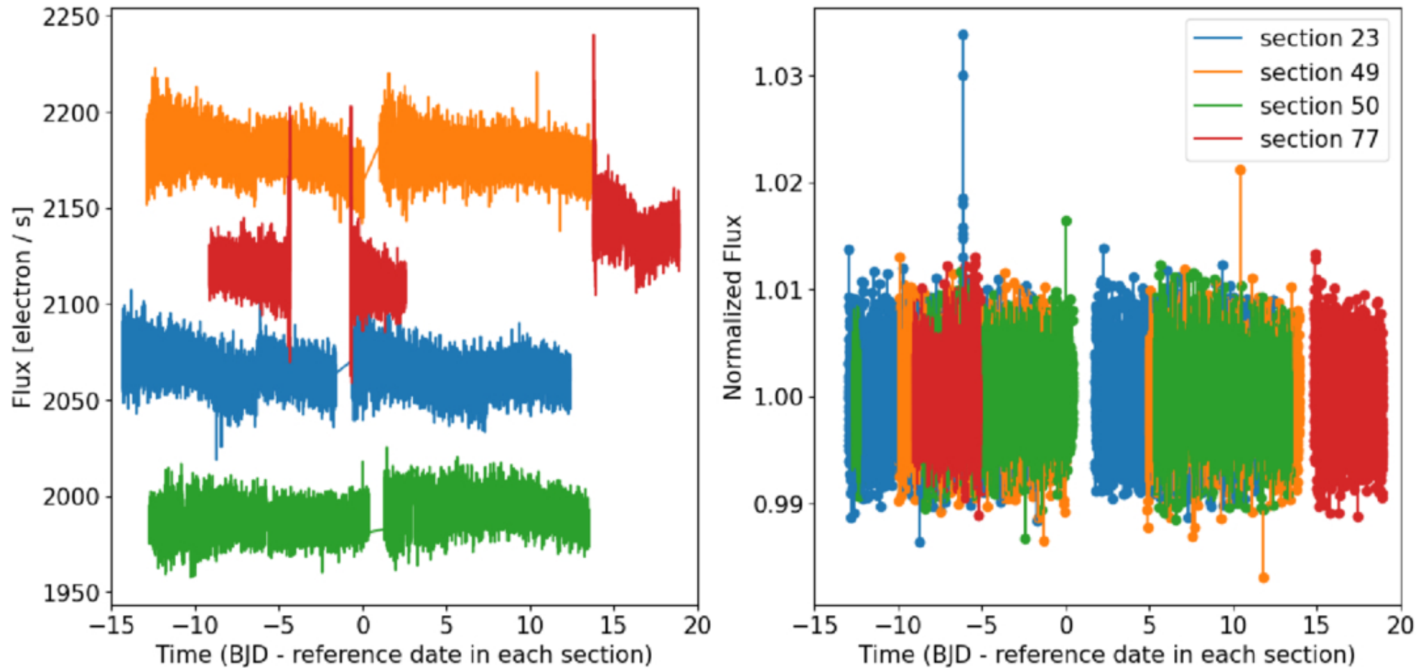
Figure 4. from Taichi Uyama et al 2025 Astron. J. 170 doi:10.3847/1538-3881/ae08b6 https://dx.doi.org/10.3847/1538-3881/ae08b6 © 2025. The Author(s). Published by the American Astronomical Society.
