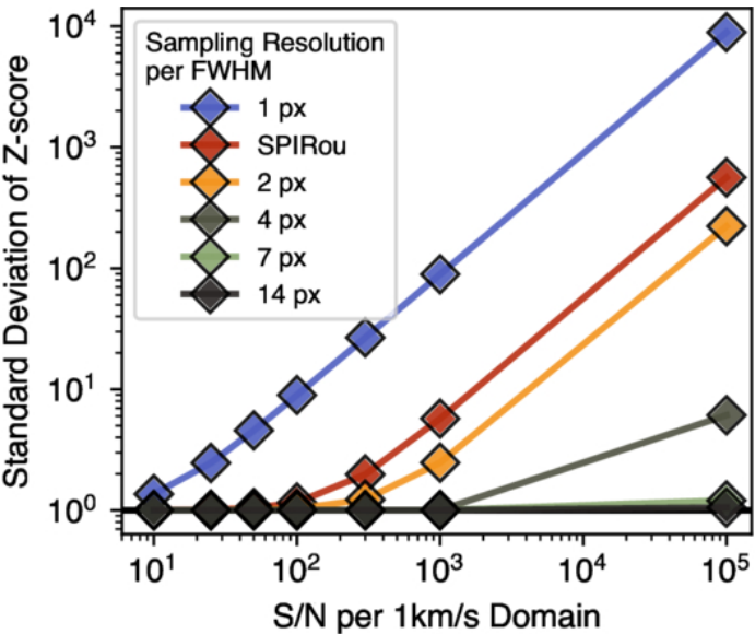
Figure 4. from Dhvani Doshi et al 2025 Astron. J. 170 doi:10.3847/1538-3881/ae08b0 https://dx.doi.org/10.3847/1538-3881/ae08b0 © 2025. The Author(s). Published by the American Astronomical Society.
