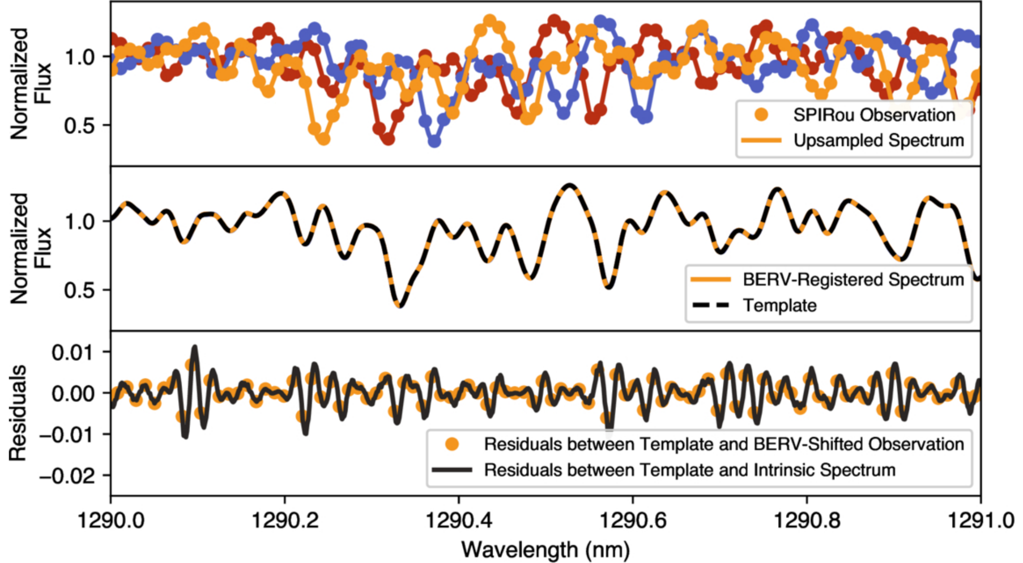
Figure 3. from Dhvani Doshi et al 2025 Astron. J. 170 doi:10.3847/1538-3881/ae08b0 https://dx.doi.org/10.3847/1538-3881/ae08b0 © 2025. The Author(s). Published by the American Astronomical Society.
