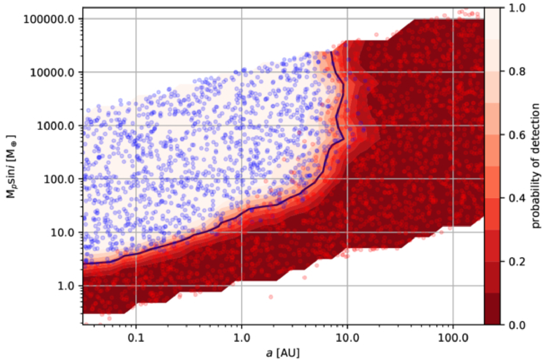
Figure 3. from Stephen R. Kane et al 2025 Astron. J. 170 doi:10.3847/1538-3881/ae089f https://dx.doi.org/10.3847/1538-3881/ae089f © 2025. The Author(s). Published by the American Astronomical Society.
