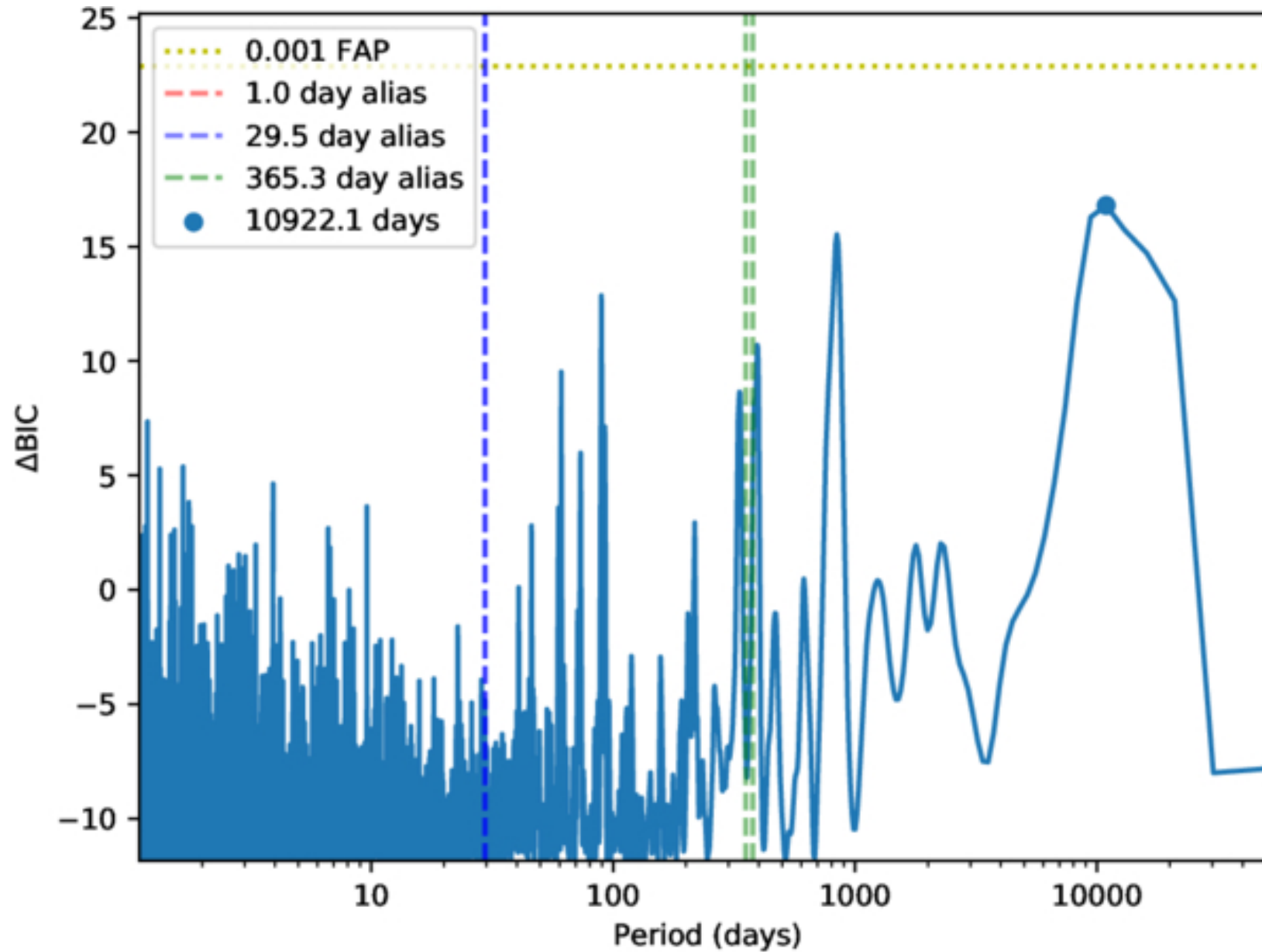
Figure 2. from Stephen R. Kane et al 2025 Astron. J. 170 doi:10.3847/1538-3881/ae089f https://dx.doi.org/10.3847/1538-3881/ae089f © 2025. The Author(s). Published by the American Astronomical Society.
