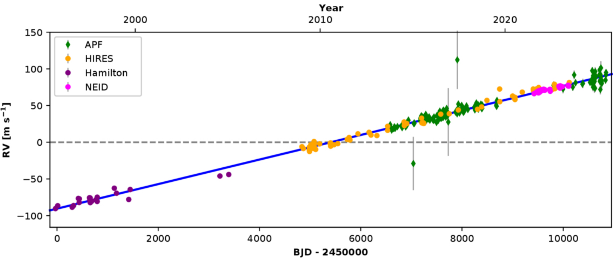
Figure 1. from Stephen R. Kane et al 2025 Astron. J. 170 doi:10.3847/1538-3881/ae089f https://dx.doi.org/10.3847/1538-3881/ae089f © 2025. The Author(s). Published by the American Astronomical Society.
