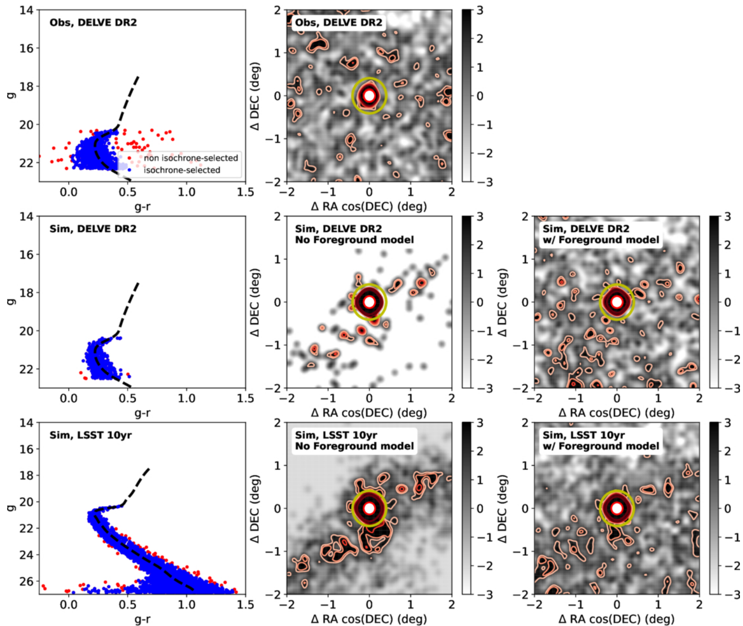
Figure 9. from A. Chiti et al 2025 Astron. J. 170 doi:10.3847/1538-3881/ae07e0 https://dx.doi.org/10.3847/1538-3881/ae07e0 © 2025. The Author(s). Published by the American Astronomical Society.
