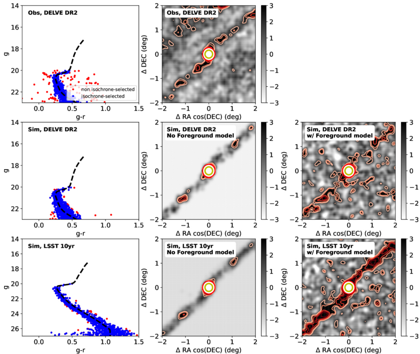
Figure 7. from A. Chiti et al 2025 Astron. J. 170 doi:10.3847/1538-3881/ae07e0 https://dx.doi.org/10.3847/1538-3881/ae07e0 © 2025. The Author(s). Published by the American Astronomical Society.
