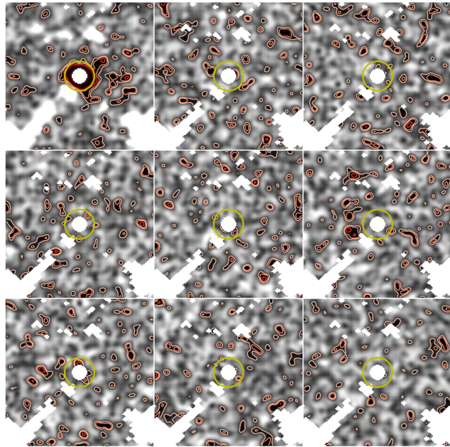
Figure 5. from A. Chiti et al 2025 Astron. J. 170 doi:10.3847/1538-3881/ae07e0 https://dx.doi.org/10.3847/1538-3881/ae07e0 © 2025. The Author(s). Published by the American Astronomical Society.
