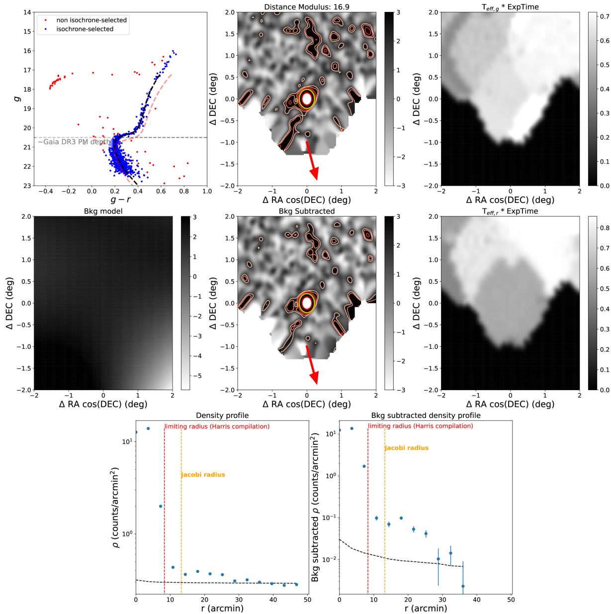
Figure 4. from A. Chiti et al 2025 Astron. J. 170 doi:10.3847/1538-3881/ae07e0 https://dx.doi.org/10.3847/1538-3881/ae07e0 © 2025. The Author(s). Published by the American Astronomical Society.
