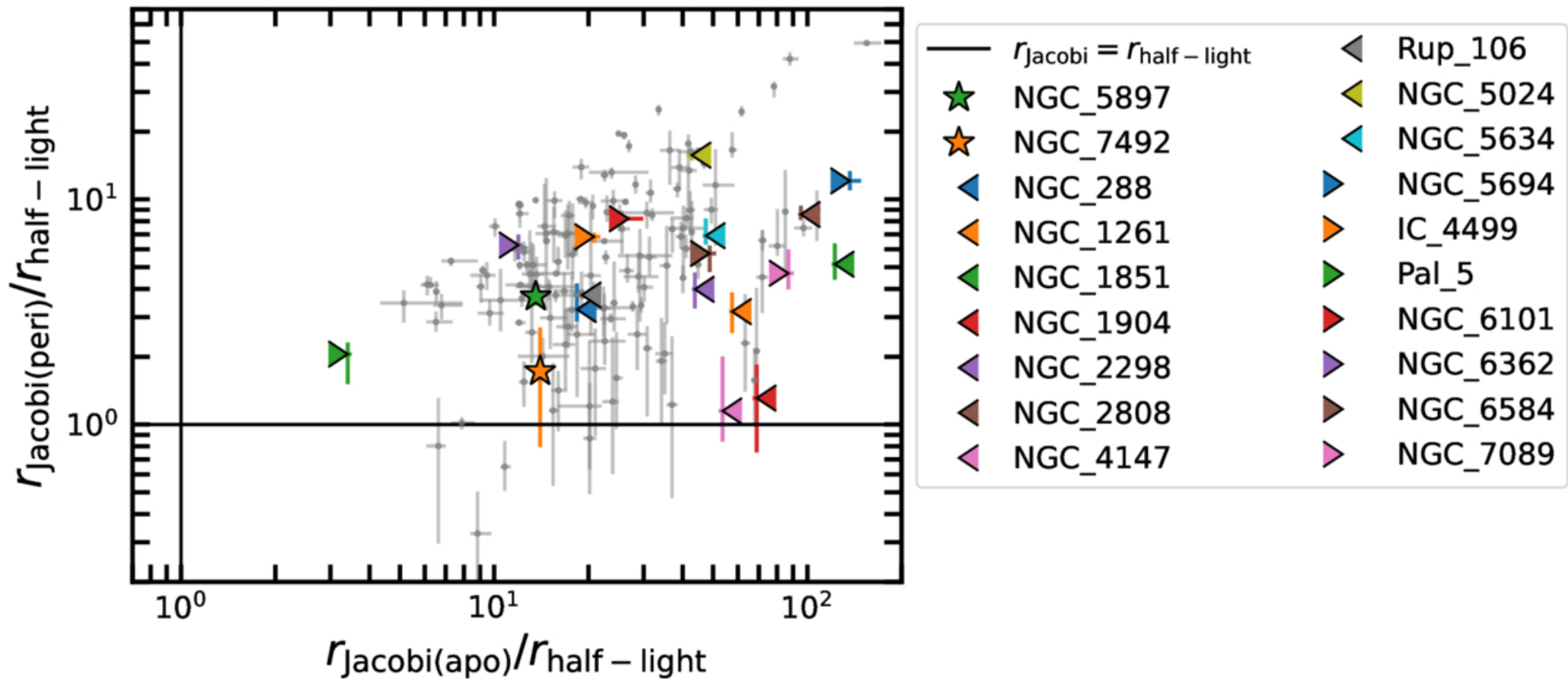
Figure 10. from A. Chiti et al 2025 Astron. J. 170 doi:10.3847/1538-3881/ae07e0 https://dx.doi.org/10.3847/1538-3881/ae07e0 © 2025. The Author(s). Published by the American Astronomical Society.
