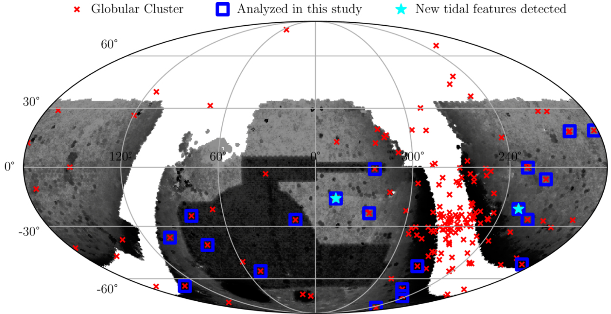
Figure 1. from A. Chiti et al 2025 Astron. J. 170 doi:10.3847/1538-3881/ae07e0 https://dx.doi.org/10.3847/1538-3881/ae07e0 © 2025. The Author(s). Published by the American Astronomical Society.
