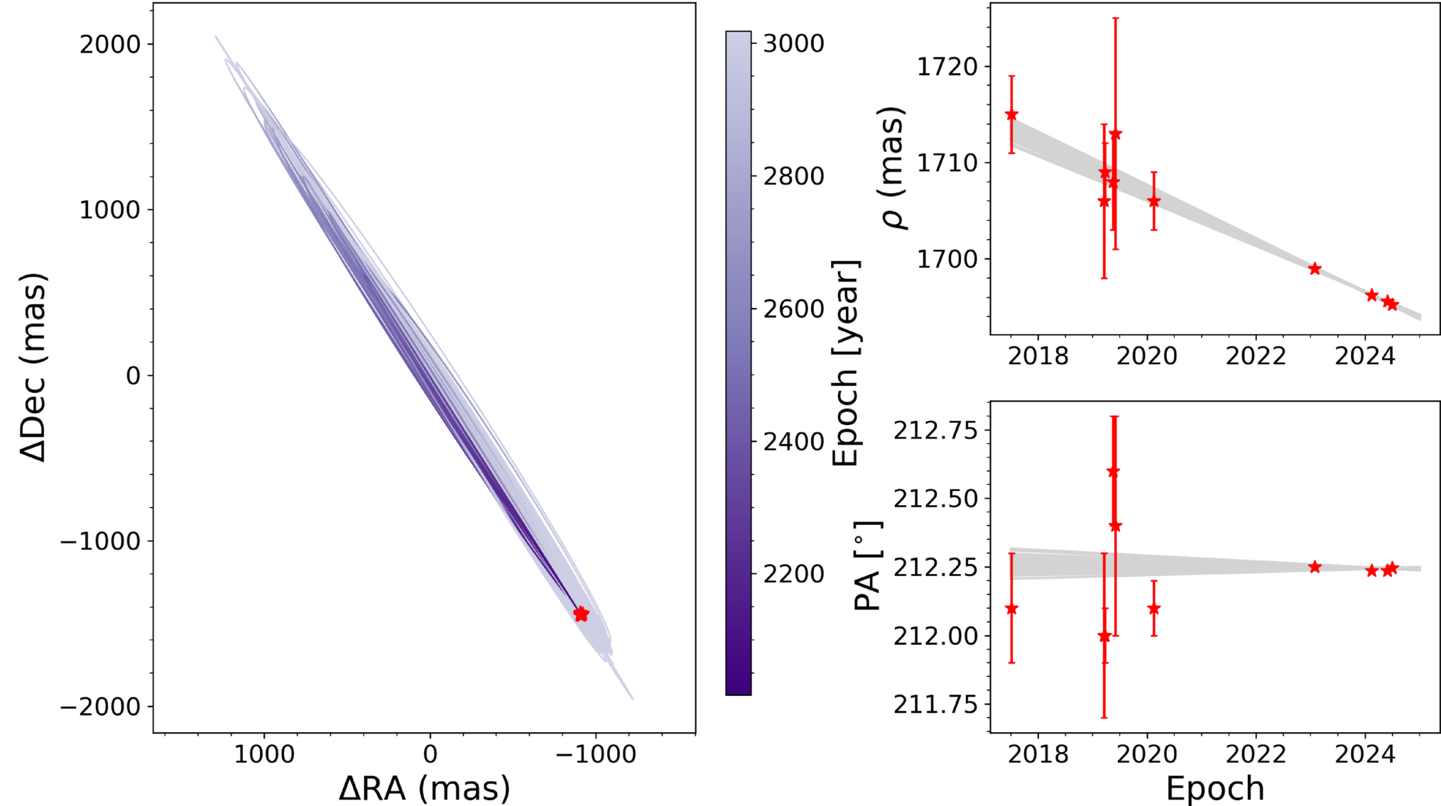
Figure 4. from Jonathan Roberts et al 2025 Astron. J. 170 doi:10.3847/1538-3881/ae07cb https://dx.doi.org/10.3847/1538-3881/ae07cb © 2025. The Author(s). Published by the American Astronomical Society.
