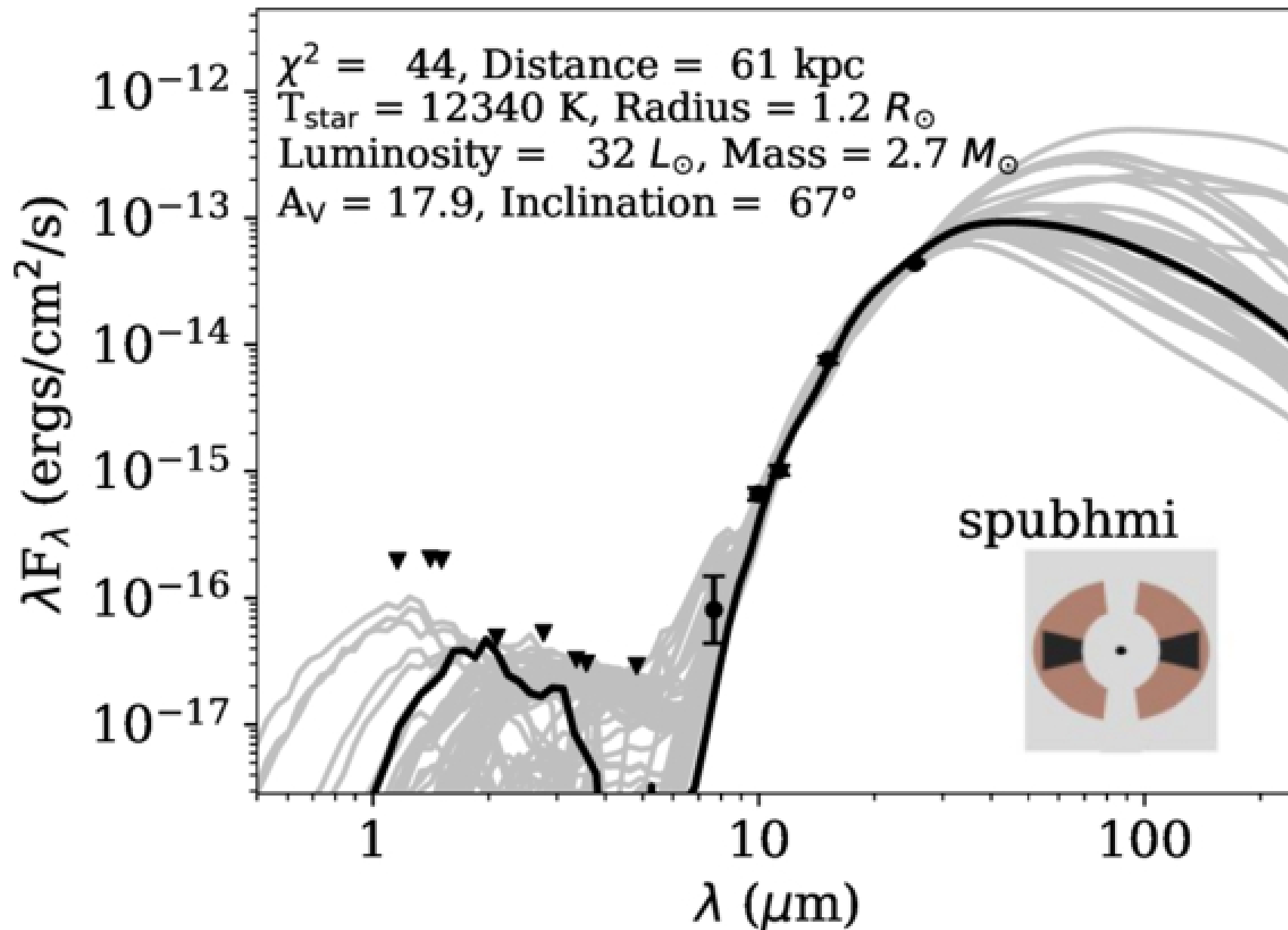
Figure 5. from Beena Meena et al 2025 Astron. J. 170 doi:10.3847/1538-3881/ae0713 https://dx.doi.org/10.3847/1538-3881/ae0713 © 2025. The Author(s). Published by the American Astronomical Society.
