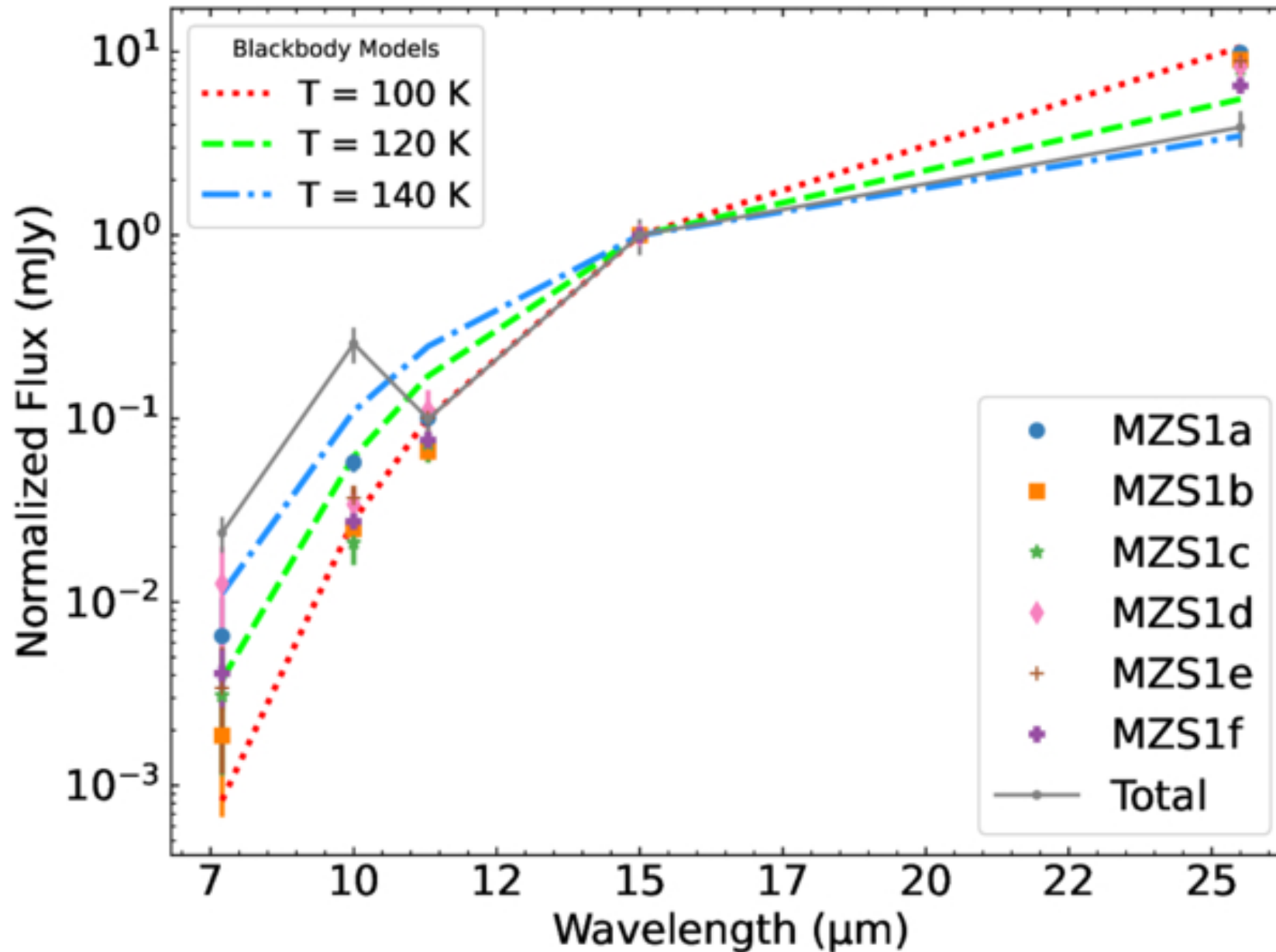
Figure 4. from Beena Meena et al 2025 Astron. J. 170 doi:10.3847/1538-3881/ae0713 https://dx.doi.org/10.3847/1538-3881/ae0713 © 2025. The Author(s). Published by the American Astronomical Society.
