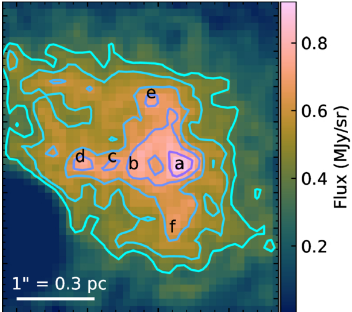
Figure 3. from Beena Meena et al 2025 Astron. J. 170 doi:10.3847/1538-3881/ae0713 https://dx.doi.org/10.3847/1538-3881/ae0713 © 2025. The Author(s). Published by the American Astronomical Society.
