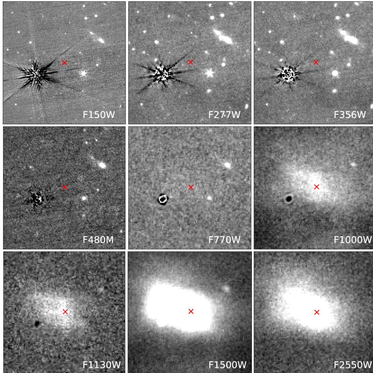
Figure 2. from Beena Meena et al 2025 Astron. J. 170 doi:10.3847/1538-3881/ae0713 https://dx.doi.org/10.3847/1538-3881/ae0713 © 2025. The Author(s). Published by the American Astronomical Society.
