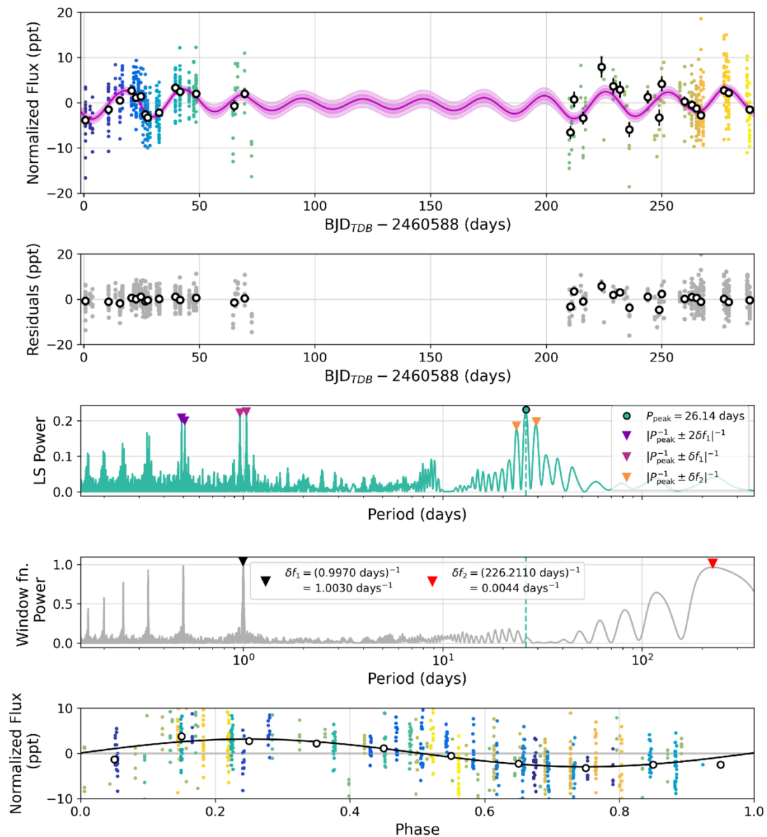
Figure 1. from Samuel W. Yee et al 2025 Astron. J. 170 doi:10.3847/1538-3881/ae070b https://dx.doi.org/10.3847/1538-3881/ae070b © 2025. The Author(s). Published by the American Astronomical Society.
