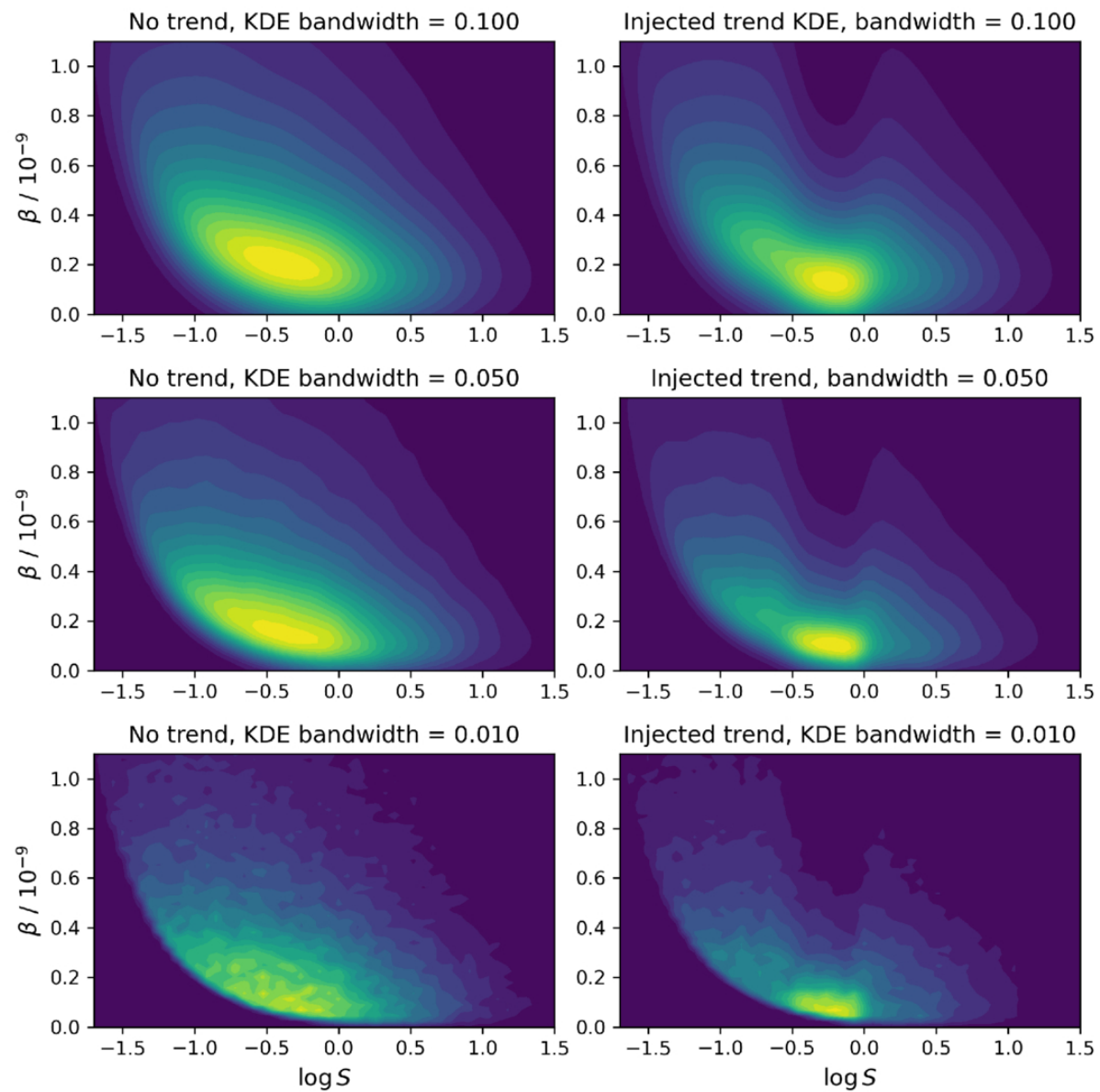
Figure 9. from Noah W. Tuchow et al 2025 Astron. J. 170 doi:10.3847/1538-3881/ae0588 https://dx.doi.org/10.3847/1538-3881/ae0588 © 2025. The Author(s). Published by the American Astronomical Society.
