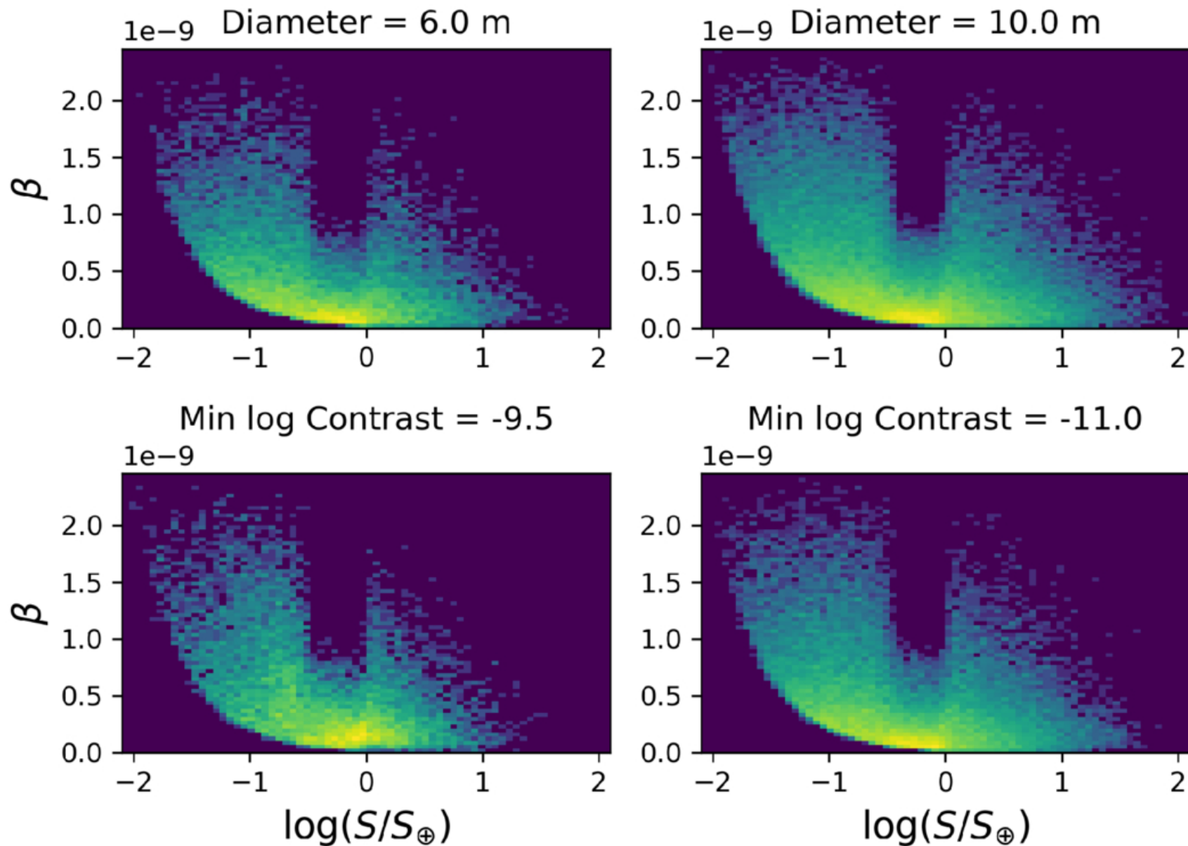
Figure 8. from Noah W. Tuchow et al 2025 Astron. J. 170 doi:10.3847/1538-3881/ae0588 https://dx.doi.org/10.3847/1538-3881/ae0588 © 2025. The Author(s). Published by the American Astronomical Society.
