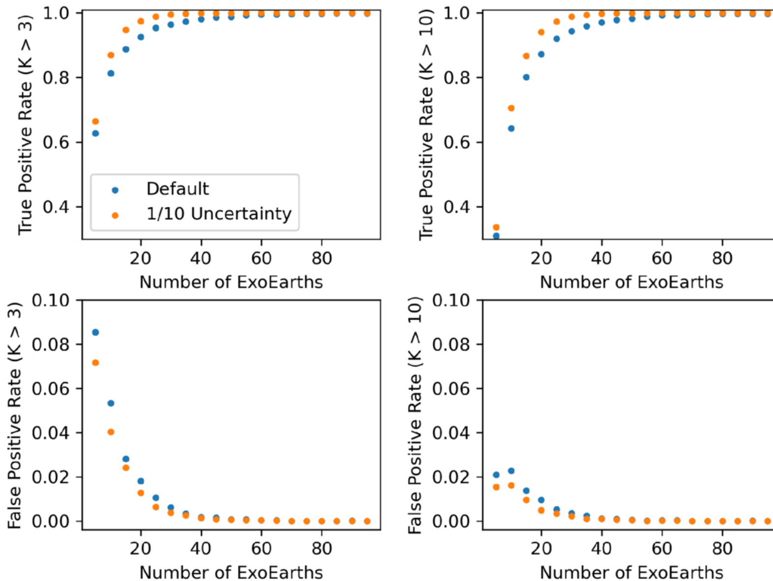
Figure 7. from Noah W. Tuchow et al 2025 Astron. J. 170 doi:10.3847/1538-3881/ae0588 https://dx.doi.org/10.3847/1538-3881/ae0588 © 2025. The Author(s). Published by the American Astronomical Society.
