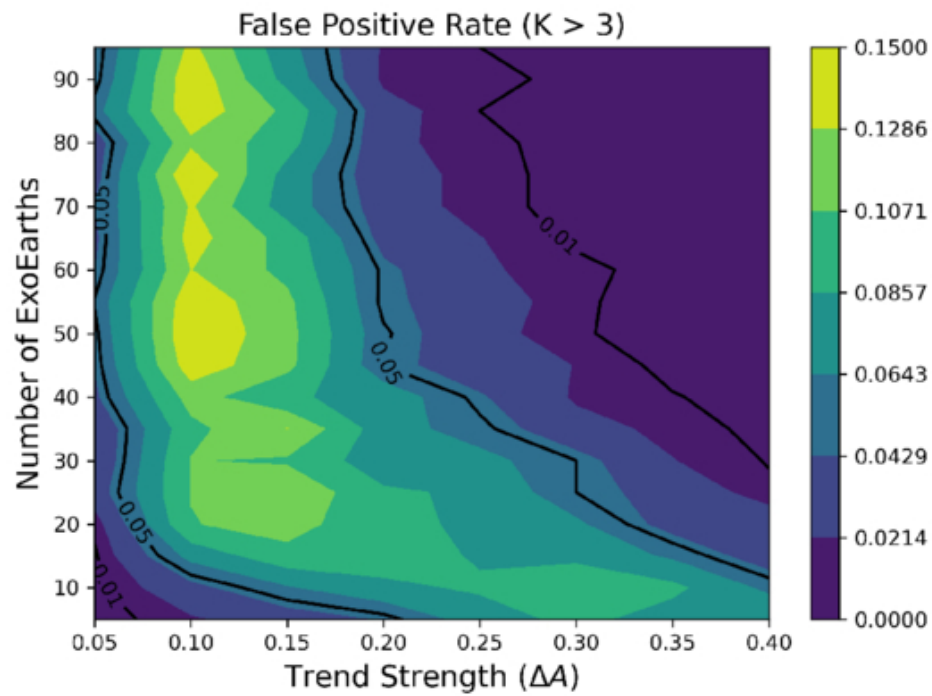
Figure 6. from Noah W. Tuchow et al 2025 Astron. J. 170 doi:10.3847/1538-3881/ae0588 https://dx.doi.org/10.3847/1538-3881/ae0588 © 2025. The Author(s). Published by the American Astronomical Society.
