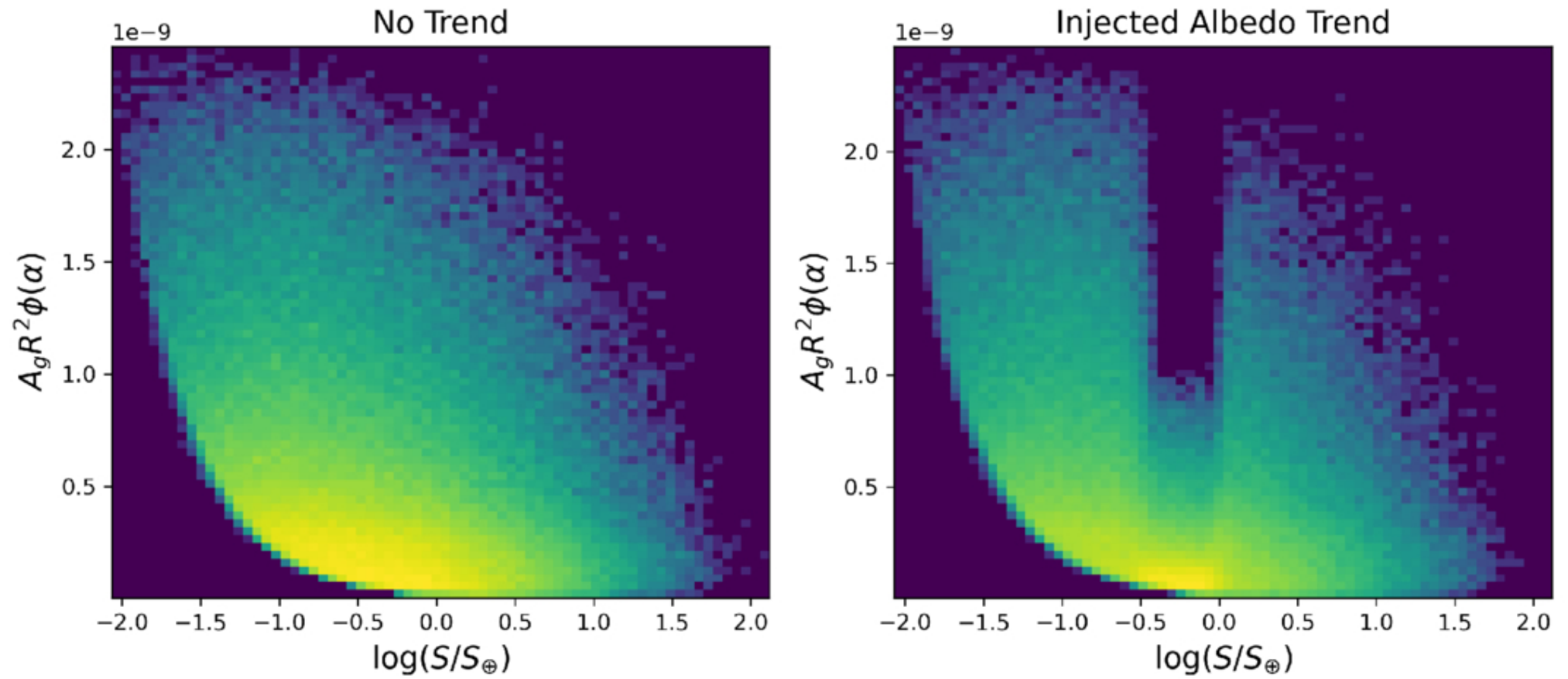
Figure 2. from Noah W. Tuchow et al 2025 Astron. J. 170 doi:10.3847/1538-3881/ae0588 https://dx.doi.org/10.3847/1538-3881/ae0588 © 2025. The Author(s). Published by the American Astronomical Society.
