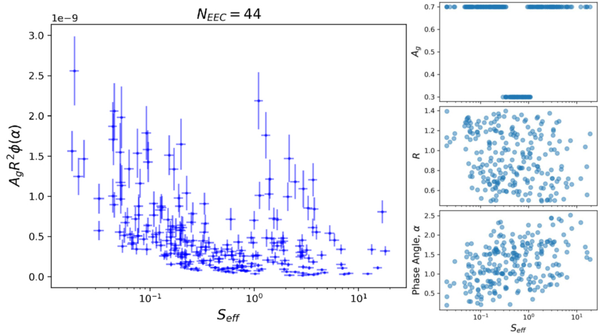
Figure 1. from Noah W. Tuchow et al 2025 Astron. J. 170 doi:10.3847/1538-3881/ae0588 https://dx.doi.org/10.3847/1538-3881/ae0588 © 2025. The Author(s). Published by the American Astronomical Society.
