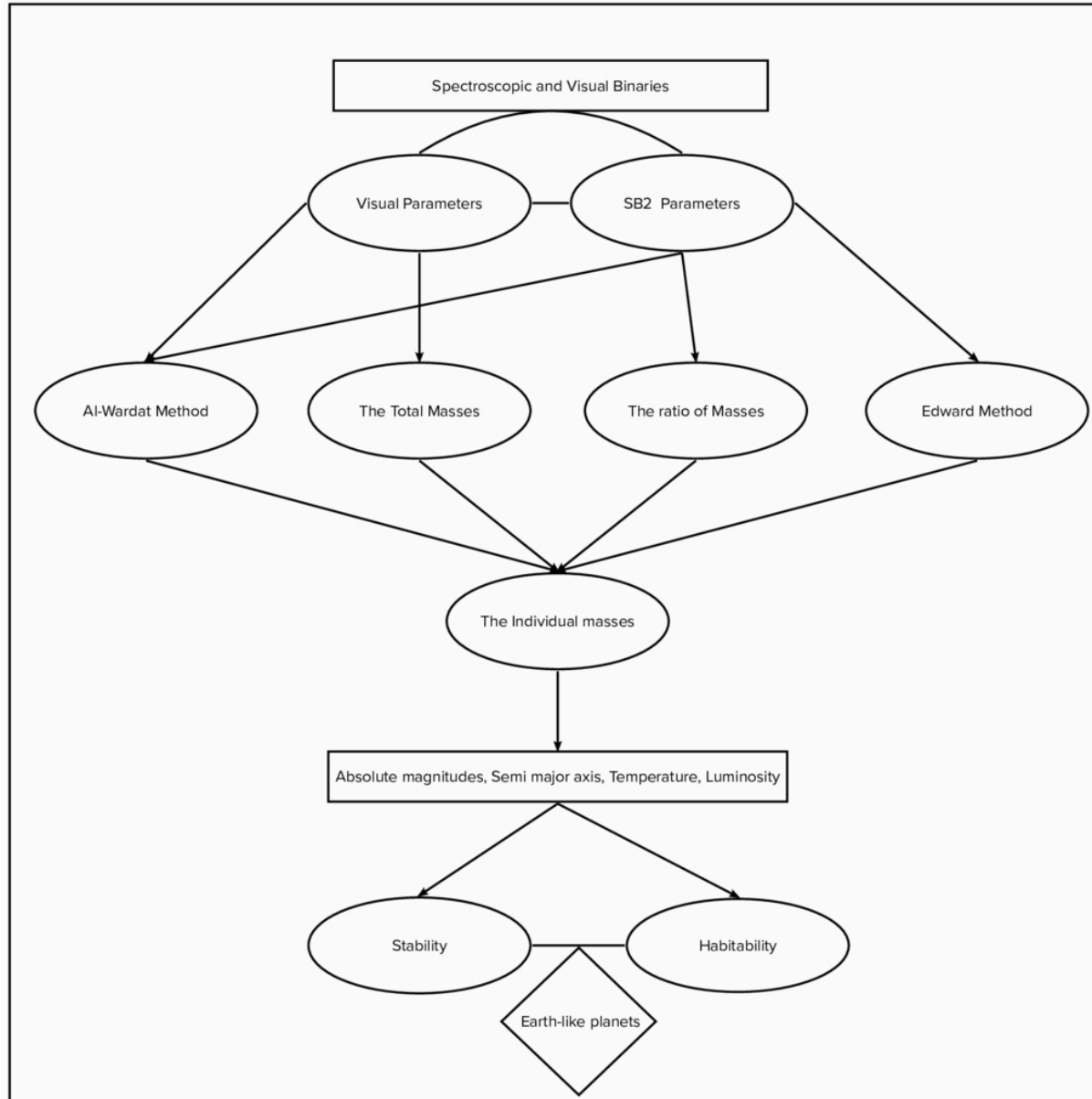
Figure 8. from Ahmad Abushattal et al 2025 Astron. J. 170 doi:10.3847/1538-3881/ae0582 https://dx.doi.org/10.3847/1538-3881/ae0582 © 2025. The Author(s). Published by the American Astronomical Society.
