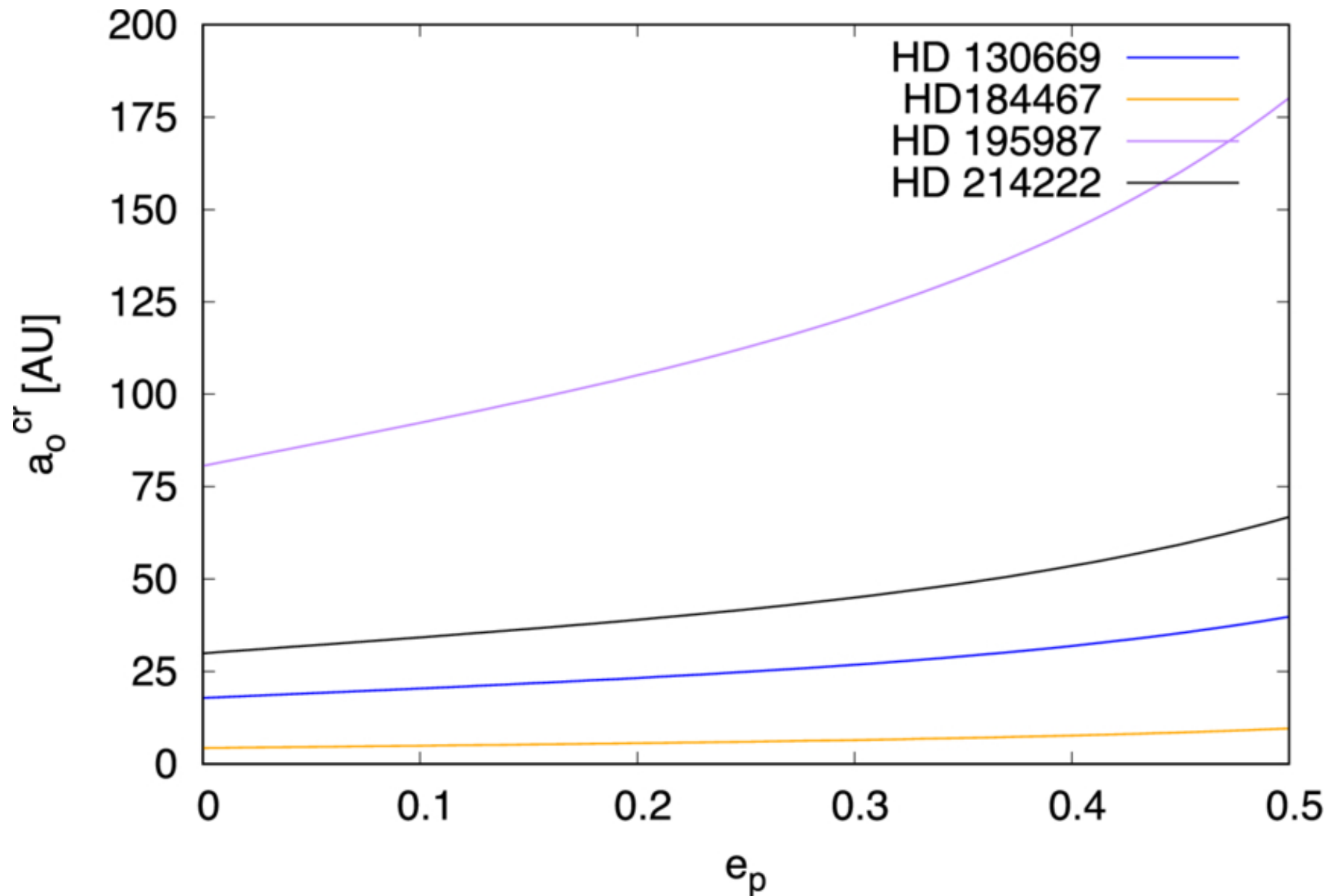
Figure 6. from Ahmad Abushattal et al 2025 Astron. J. 170 doi:10.3847/1538-3881/ae0582 https://dx.doi.org/10.3847/1538-3881/ae0582 © 2025. The Author(s). Published by the American Astronomical Society.
