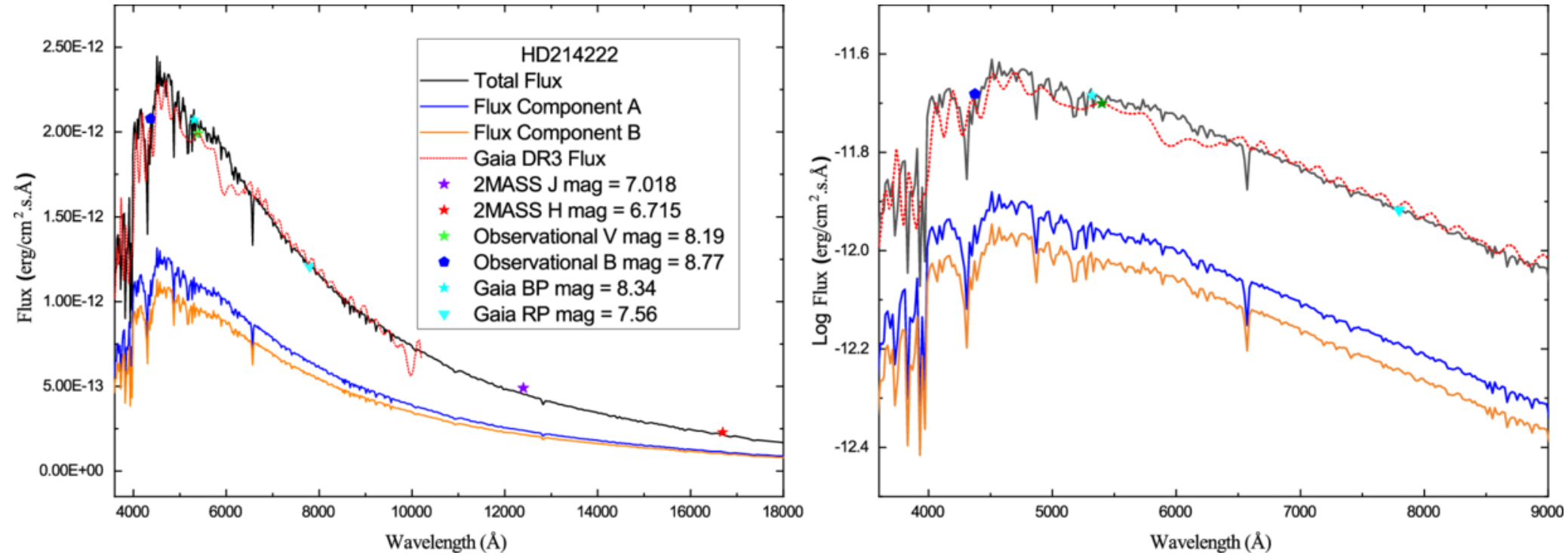
Figure 4. from Ahmad Abushattal et al 2025 Astron. J. 170 doi:10.3847/1538-3881/ae0582 https://dx.doi.org/10.3847/1538-3881/ae0582 © 2025. The Author(s). Published by the American Astronomical Society.
